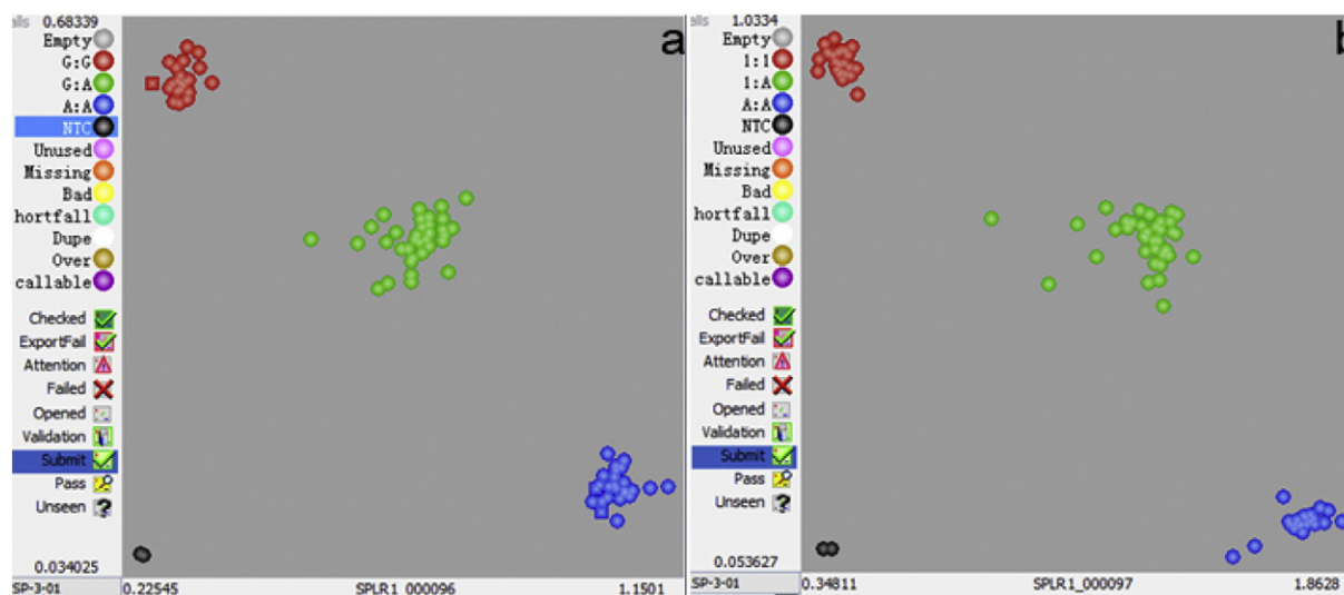
Fig. 2. Genotyping results of AhFAD2A (a) and AhFAD2B (b) by KASP. The scatter plot with axes x and y represents allelic discrimination of FAD2A or FAD2B genotypes. The red, green and blue dots represent the mutant homozygous, heterozygous and wild-type homozygous, respectively.
