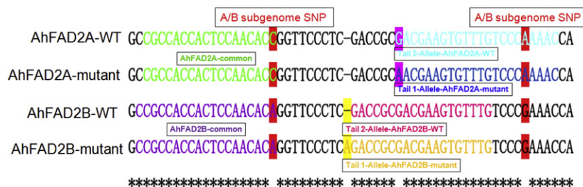
Fig. 1. Locations of genetic mutations and primer design in both AhFAD2A and AhFAD2B alleles. Different primer sites were shown with different colors. All primer sequences were shown in Table 1.
