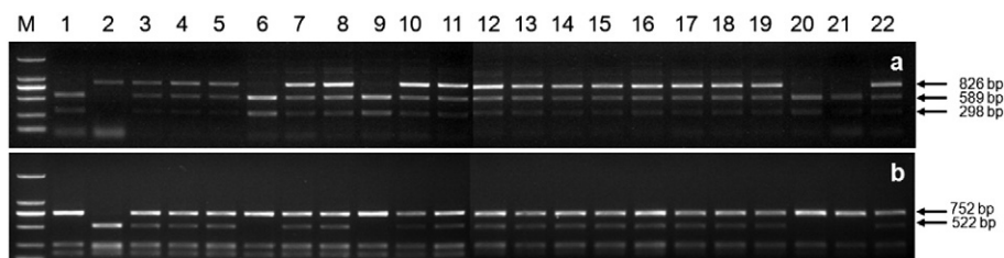
Fig. 3. Genotyping results of AhFAD2A and AhFAD2B by CAPS. (a) Hpy99I digestion of PCR products; (b) Hpy188I digestion of PCR products. M referred to DL5000 DNA Marker; Lane 1 and Lane 2 showed the genotypes of Huayu31 and Kainong176, respectively; Lanes 3–22 showed the genotypes of 20 F_1 seeds, respectively.
