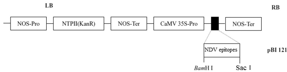
Fig. 2. Schematic structure of the recombinant plasmid pBI121-NDV epitopes for Agrobacterium -mediated transformation of tobacco plant. The DNA sequence encoding NDV epitope was cloned the downstream of the CaMV 35S promoter of a binary plasmid pBI 121.
