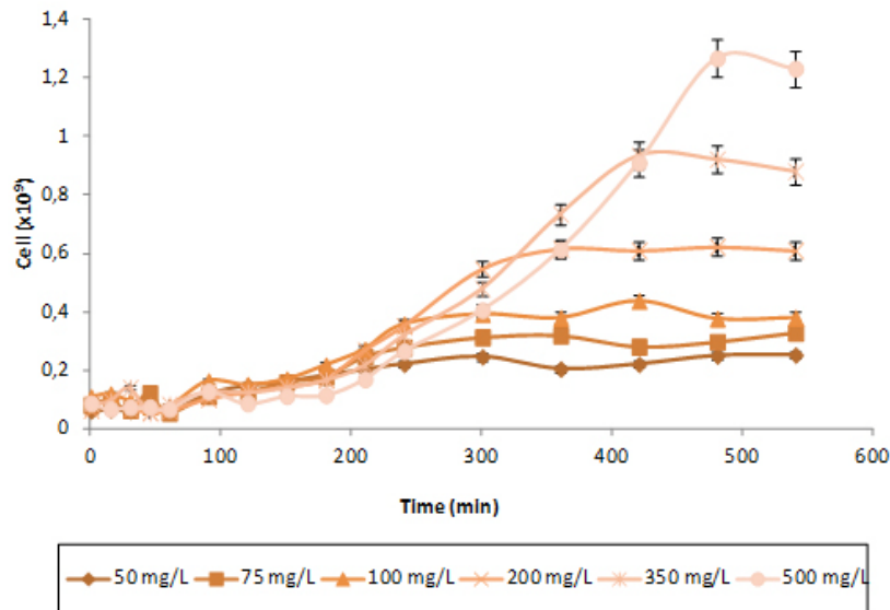
Fig. 4 Cell growth at different initial concentrations of o-cresol.
