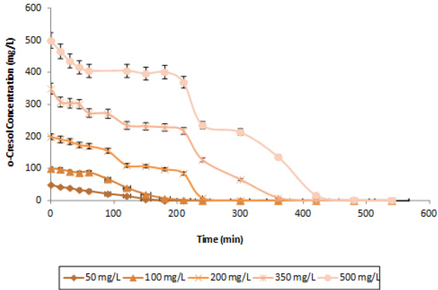
Fig. 3 Biodegradation of o-cresol at different initial concentrations of o-cresol.
