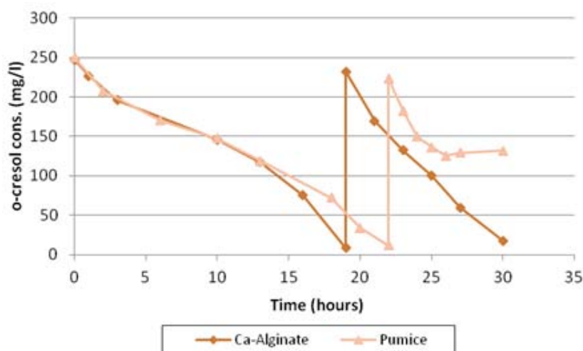
Fig. 8 o-cresol biodegradation comparison between packed bed reactor cycles.
