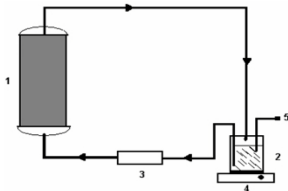
Fig. 1 Batch recirculation system operated bioreactor: (1) reactor, (2) feed reservoir, (3) peristaltic pump, (4) magnetic stirrer, (5) sampling.
