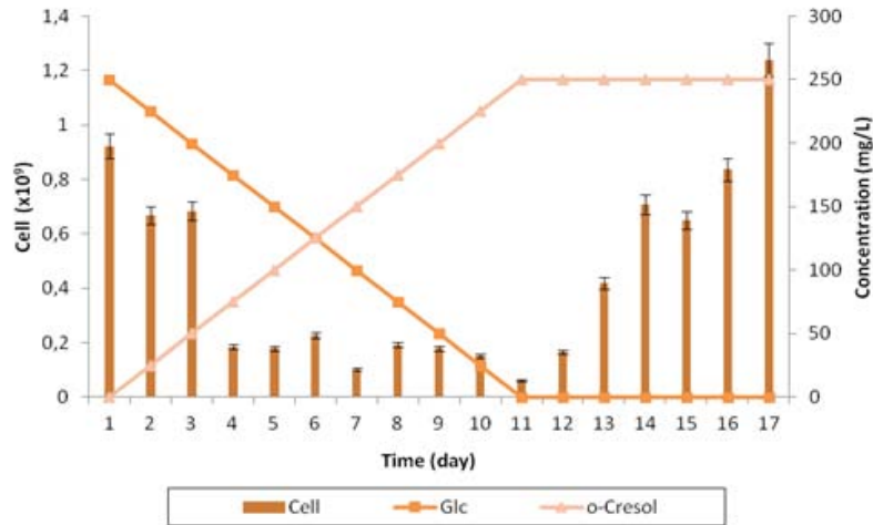
Fig. 2 Adaptation process of P. putida .
