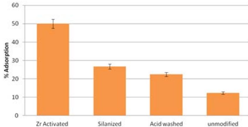
Fig. 7 Cell adsorptions of different treated pumices.
