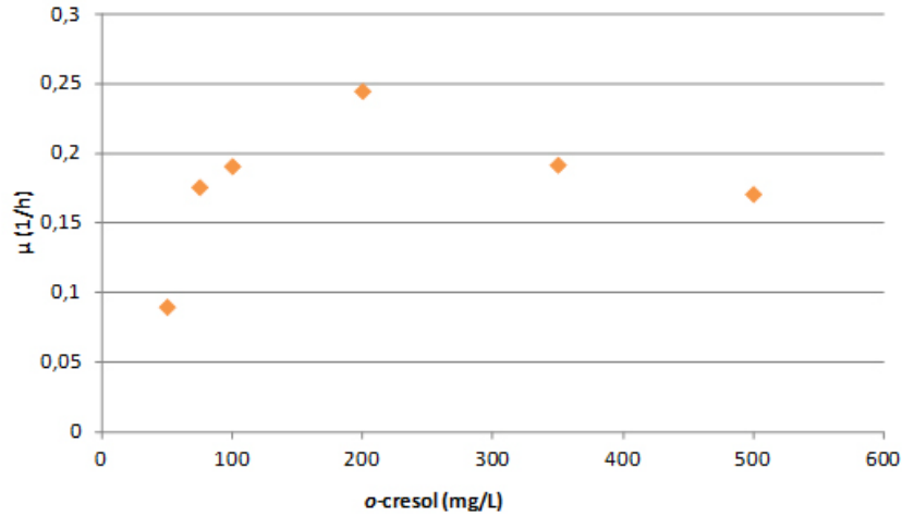
Fig. 5 Haldane's growth model fitted to results of batch growth experimental data to determine kinetic parameters.
