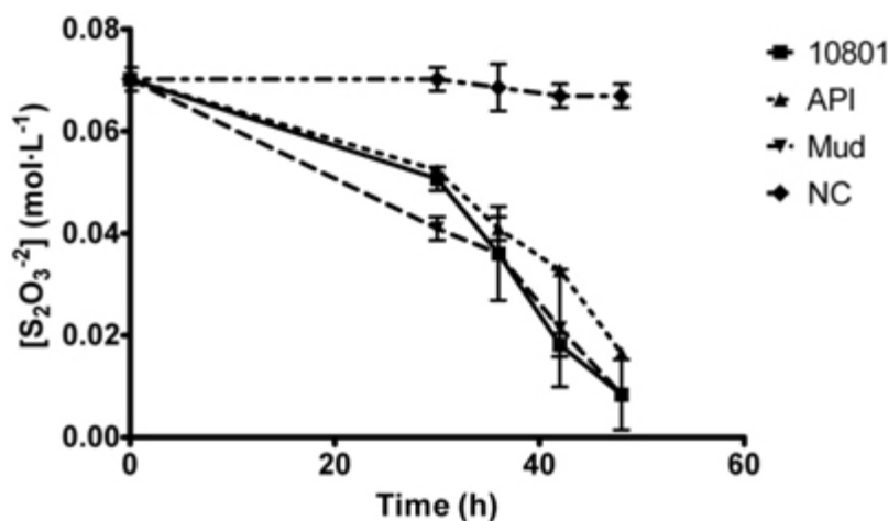
Fig. 2 Thiosulphate consumption (mol L -1 ) vs Time (hrs) of strains isolated in this study and the T. thioparus ATCC 10801 strain at 24°C. 10801, ATCC 10801 strain; API, water separator strain; MUD, sludge strain; NC, Negative Control (non inoculated). [S 2 O 3 -2 ]: Thiosulphate concentration.
