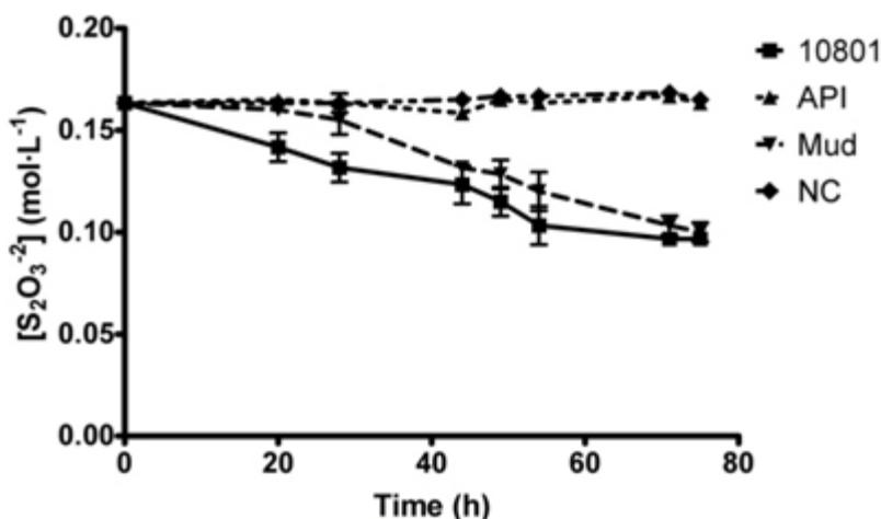
Fig. 3 Thiosulphate consumption ( \text{mol L}^{-1} ) vs Time (hrs) of strains isolated in this study and the T. thiooparus ATCC 10801 strain at 30°C. 10801, ATCC 10801 strain; API, water separator strain; MUD, sludge strain; NC, Negative Control (non inoculated). [\text{S}_2\text{O}_3^{2-}] : Thiosulphate concentration.
