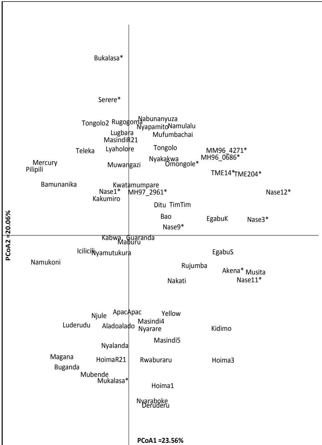
Figure 1. Principle coordinates analysis from dissimilarity coefficients of 66 cassava accessions (elite accessions are marked with asterisks).
