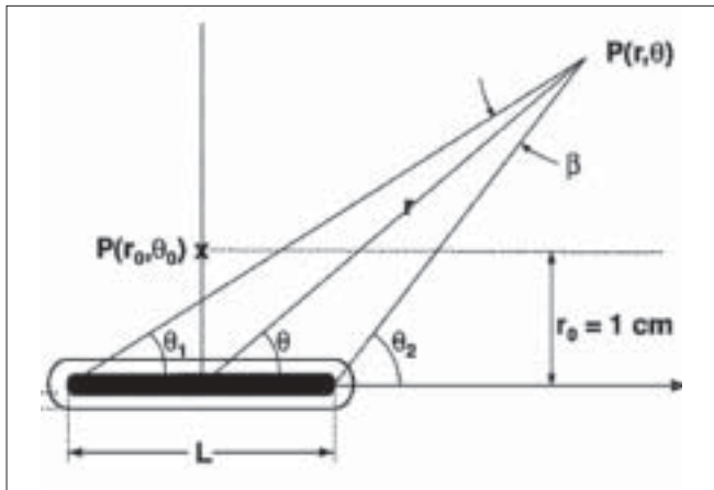
Figure 1: Radial and angular co-ordinate definition with respect to source used in AAPM TG-43 formalism
