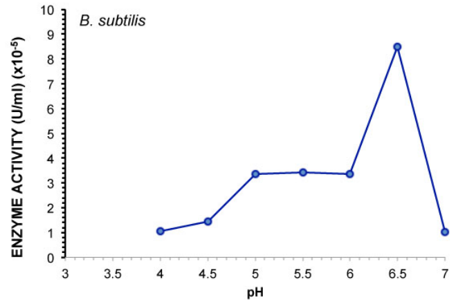
Figure 5: Effect of pH on lignin peroxidase activity produced by B. subtilis . The optimum pH of lignin peroxidase enzyme produce by B. subtilis was at pH 6.5 with activity of 8.50 \times 10^{-5} U/ml. pH values below or above this optimum values showed reduced lignin peroxidase activity.
