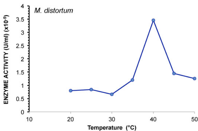
Figure 4: Effect of temperature on lignin peroxidase activity produced by M. distortum . The optimum temperature of M. distortum , was at 40 °C with activity of 3.45 \text{ U/ml} \times 10^{-5} , temperature above and below 40 °C showed low lignin peroxidase activity.
