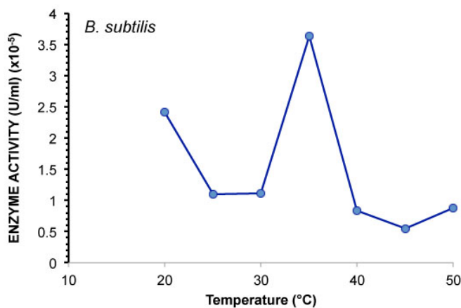
Figure 3. Effect of temperature on lignin peroxidase activity produced by B. subtilis . The optimum temperature of B. subtilis was at 35 °C with activity of 3.63 \times 10^{-5} U/ml, temperature above and below 35 °C showed low lignin peroxidase activity.
