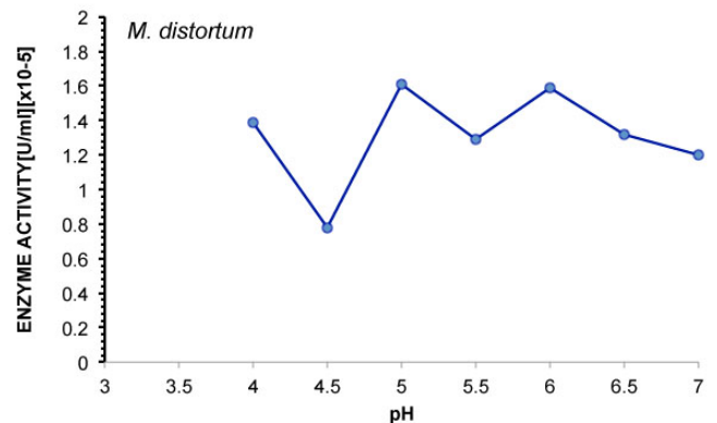
Figure 6: Effect of pH on lignin peroxidase activity produced by M. distortum . The optimum pH of lignin peroxidase enzyme produced by M. distortum was at pH 5 with activity of 1.61 \text{ U/ml} \times 10^{-5} . pH values below or above this optimum values showed reduced lignin peroxidase activity.
