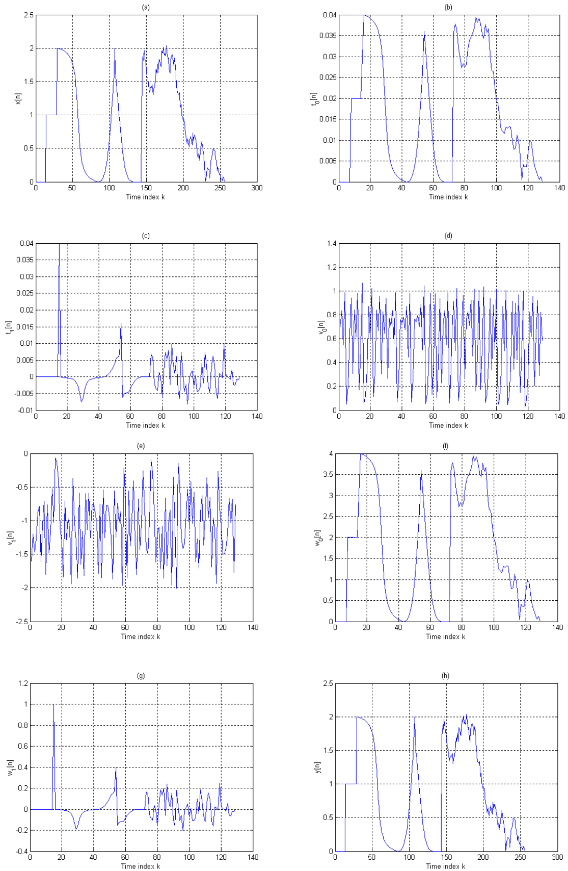
Figure 2. A one dimensional test signal [Mallat, 1992]. (a) x[n] . (b) t_0[n] . (c) t_1[n] . (d) v_0[n] . (e) v_1[n] . (f) w_0[n] . (g) w_1[n] . (h) y[n] .
