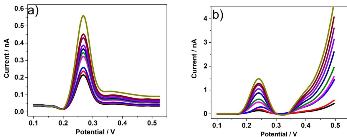
Figure 6. DPSV (background subtracted) at the \mu\text{TIES} array in different sample matrices without additional electrolyte. Response from 0.1 to 1.0 nM \text{PFOS}^- a) for drinking water, b) for seawater.
