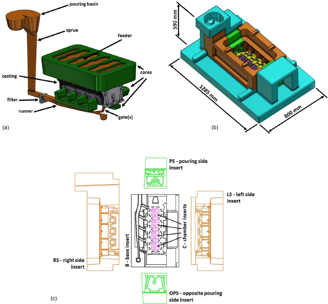
Fig. 4. CAD models of (a) the casting cavities and cores, of (b) the complete die and of (c) its inserts in an opened view.
