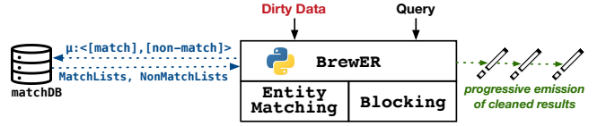
Figure 3: BrewER overview.
