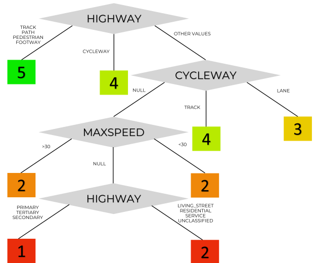
Fig. 4. Security levels decision tree.
