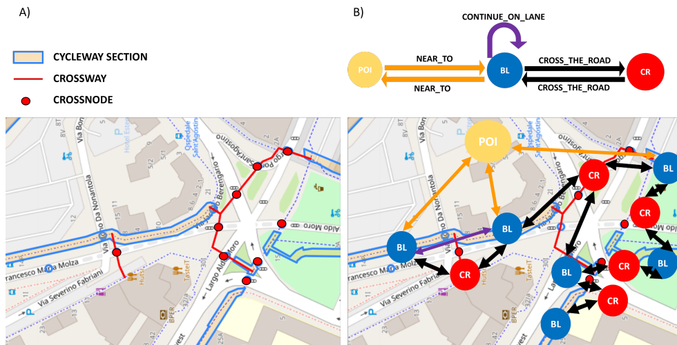
Fig. 7. Physical elements on map and the derived graph model.
