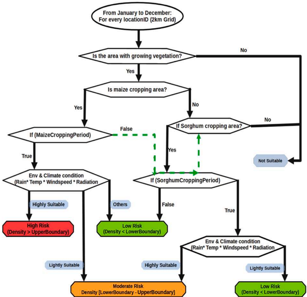
Fig. 7. Summary of the ‘rules’ for estimating the Fall armyworm (FAW) density level of infestation. Maize and sorghum are considered the main host plants of the pest. The green arrow shows the algorithmic iterations if the timing was within the sorghum planting period and cropping area.
