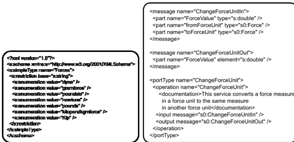
Figure 6: Improved WSDL document and XSD file
