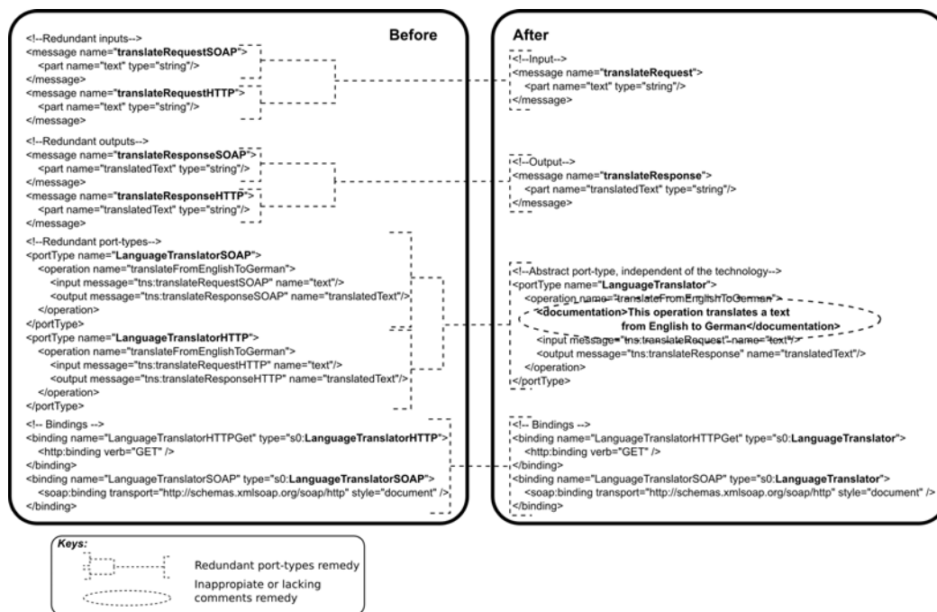
Figure 3: Remedying a WSDL document: before and after eradicating anti-patterns.
