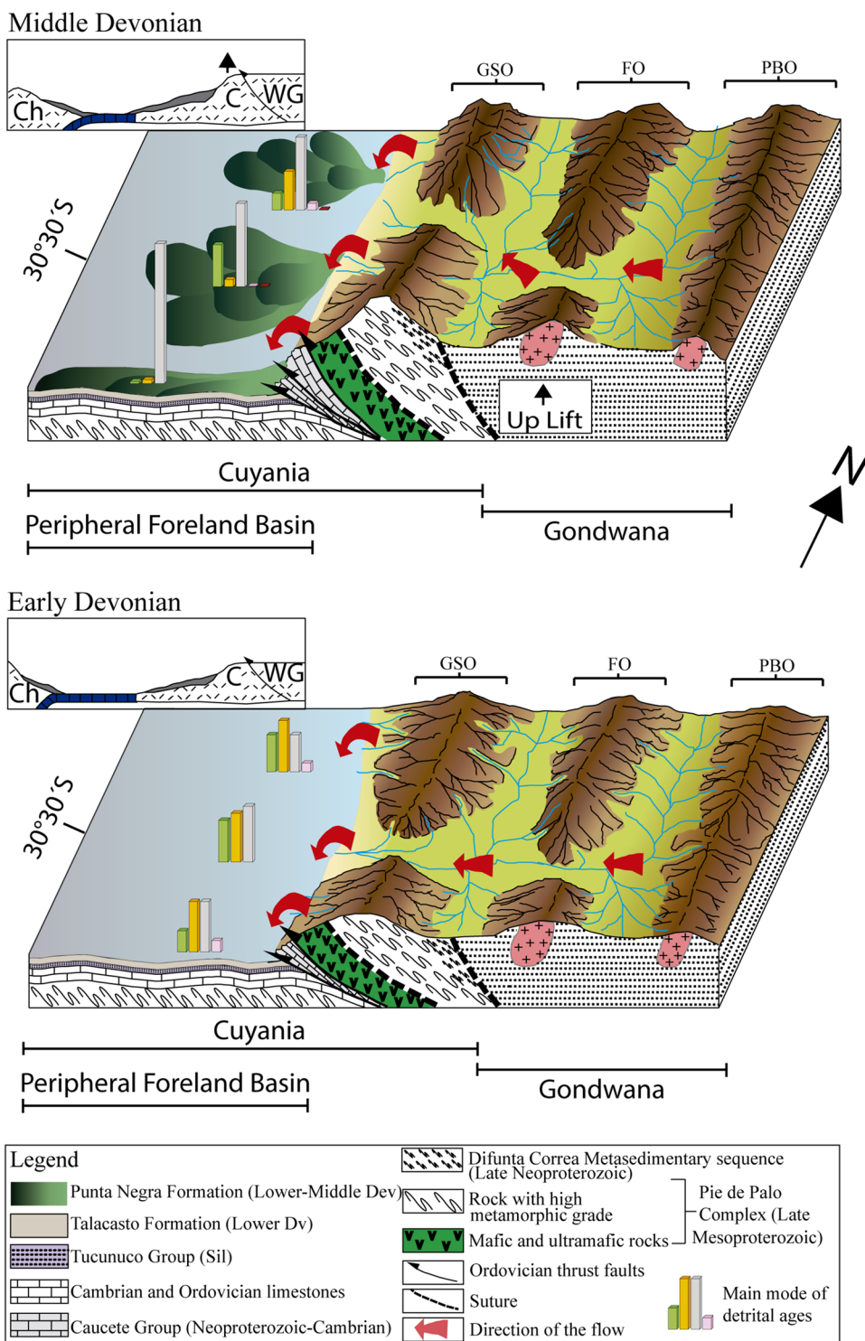
Fig. 18 Block diagram showing the Devonian distribution for the Gualilán Group, a peripheral foreland basin located westwards of the western margin of Gondwana developed in the vicinity of the Grenvillian-Sunsas orogen which is the most likely source of detritus. The highlands located in the East comprise the Grenvillian-Sunsas (GSO), Pampean–Brazilian (PBO) and Famatinian (FO) orogens. The colours of the histograms are related to the orogenic cycle from which the detrital zircon derived (see Fig. 16), whereas the height is proportional to the percentage of each of them. Ch Chilena Terrane, C Cuyania Terrane, WG Western Gondwana. Top left insets show the subduction between western Gondwana (with Cuyania already accreted) and Chilena terrane
