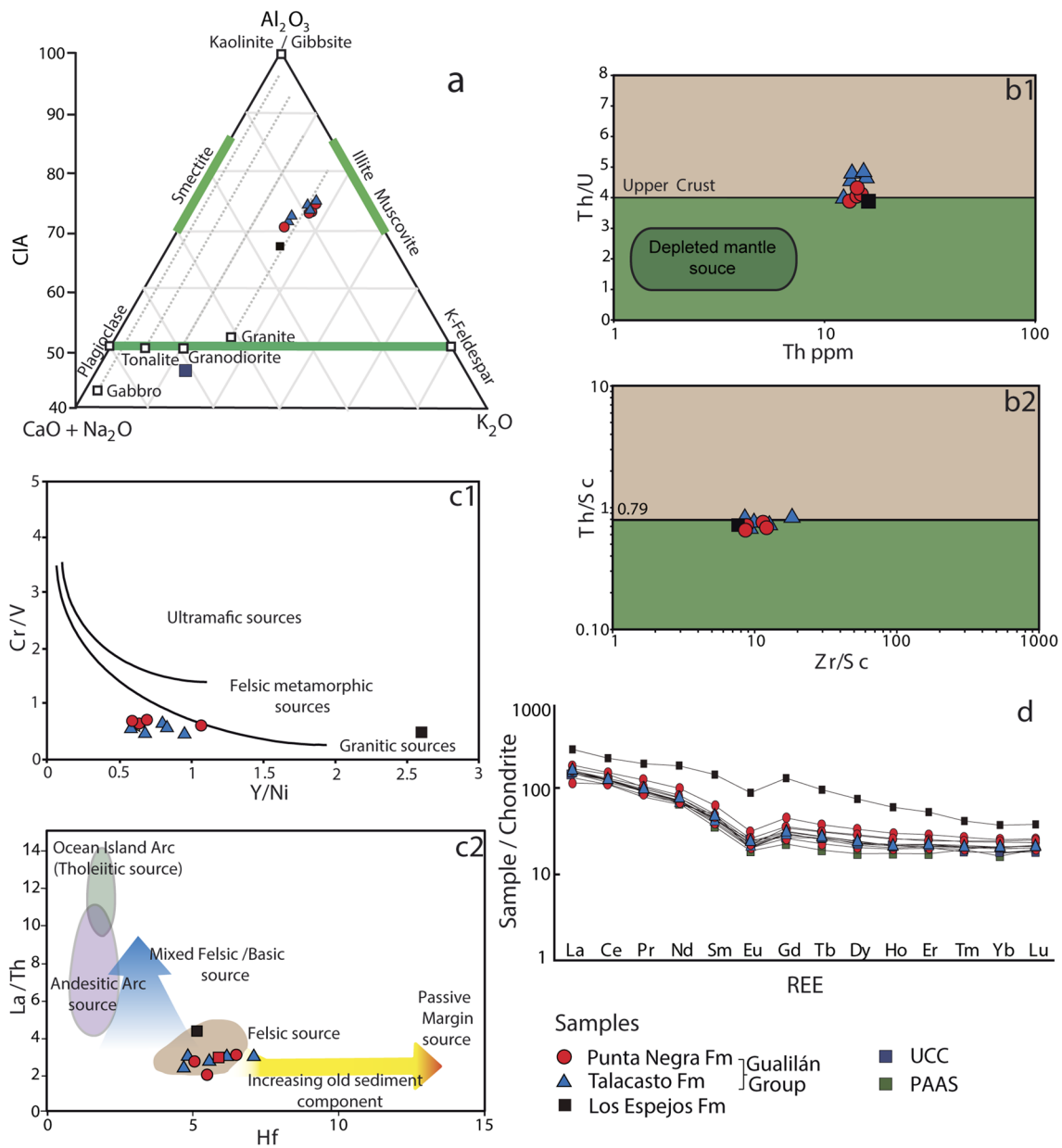
Fig. 10 a A-CN-K diagram for the Gualilán Group. Idealized mineral compositions and crystalline rocks values are according to Taylor and McLennan (1985). Dotted lines indicate the predicted weathering trend for the average parental rock compositions (Nesbitt and Young 1984, 1989). Note that the lower part of the diagram with A < 40 is not shown. The left side of the figure shows the range of CIA values. b1 Th/U vs. Th diagram (after McLennan et al. 1993). b2 Th/Sc vs. Zr/Sc diagram (after McLennan et al. 2003). c1 Cr/V vs. Y/Ni diagram (after Hiscott 1984). Upper and lower curves represent the mixing lines of ultramafic ( Cr/V = 45 ; Y/Ni = 0.001 ), felsic metamorphic ( Cr/V = 1.23 ; Y/Ni = 1.02 ), and granitic ( Cr/V = 0.25 ; Y/Ni = 2.33 )
