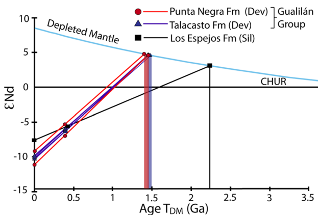
Fig. 11 \epsilon_{Nd} vs. age. Samples were compared to CHUR (Chondritic Uniform Reservoir)
