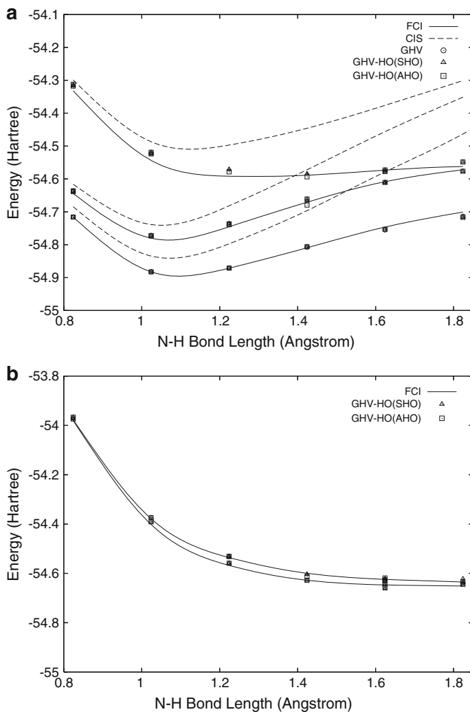
Fig. 4 Energy values (in Hartree) for a the ground state and first two doublet excited states and b the first two quartet excited states of the totally-symmetric bond stretching mode of \text{NH}_2 as functions of the N-H bond length, respectively. The solid and dashed curves denote the FCI and CIS energy curves respectively, while triangles , squares and circles denote energies computed by means of the GHV-HO method
