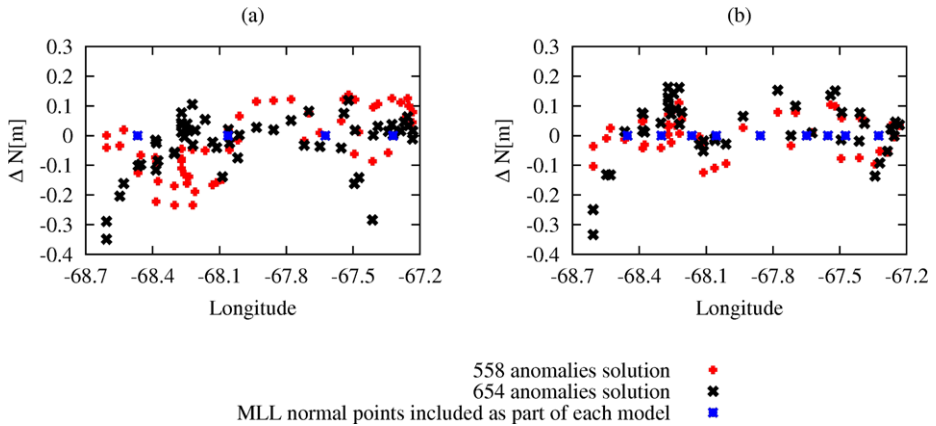
Fig. 6 Both panels depict the differences obtained after the comparison of the combined geoid models with the remaining values of MLL data, which were not included in the model. Both were based on the information of 58 GPS/levelling points and a certain number of reduced gravity anomalies and MLL normal points. Two solutions are shown in each graphic: one which includes 654 reduced gravity anomalies ( black ) and other with 558 reduced gravity anomalies. In (a) 4 MLL normal points served as reference while in (b) the number of considered MLL observations was 9, not also distributed along the east-west axis, but considering the north-south direction as well
