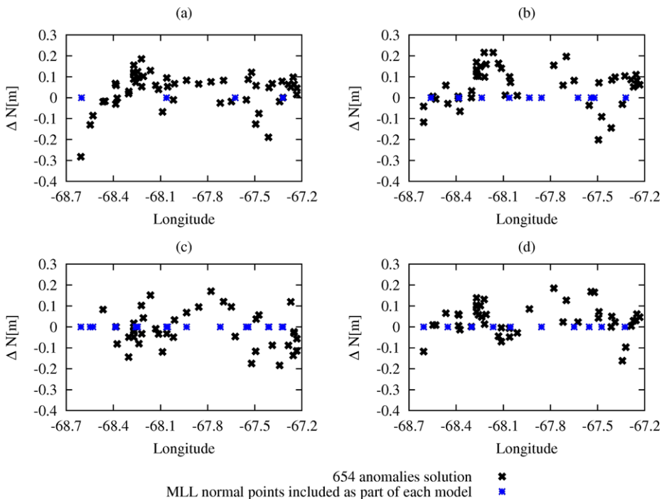
Fig. 3 The four panels depict the differences obtained after the comparison of 4 geoid models with observed geoid undulations at the sites of the remaining MLL observation, which were not introduced in the model. The four geoid models are based on the same set of 654 reduced gravity anomalies and the information of 58 GPS/levelling points, but they include different subsets of MLL normal points considered as reference: (a) 4 MLL normal points; (b) 10 MLL normal points; (c) 18 MLL normal points; (d) 10 MLL normal points as reference not also distributed along the east-west axis as case (b), but considering the north-south direction
