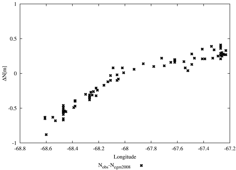
Fig. 5 Comparison of the EGM2008 geopotential model with MLL observations. The differences between model and observations are shown along the direction of the main axis of Fagnano Lake
