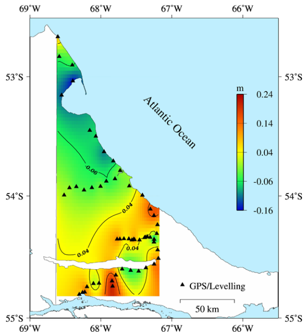
Fig. 4 EGM2008 evaluation at GPS/levelling points ( black triangles ). The colour scales represents geoid undulation differences; contour interval: 10 cm
