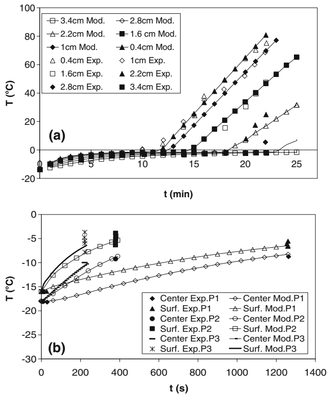
Fig. 3 a Model predictions ( continuous line + symbol ) for microwave thawing of ground beef and experimental data obtained by Taher and Farid (2001) in different internal positions ( symbols ), P_o=650 W. b Temperature profiles predicted by the numerical model and experimental results obtained in tylose bricks ( symbols ; Chamchong and Datta (1999)) for 2D heat transfer, for P_o=25,400 W/m 2 , affected by different reducing percentages: P_1=2,450 W/m 2 , P_2=12,700 W/m 2 , P_3=17,780 W/m 2
