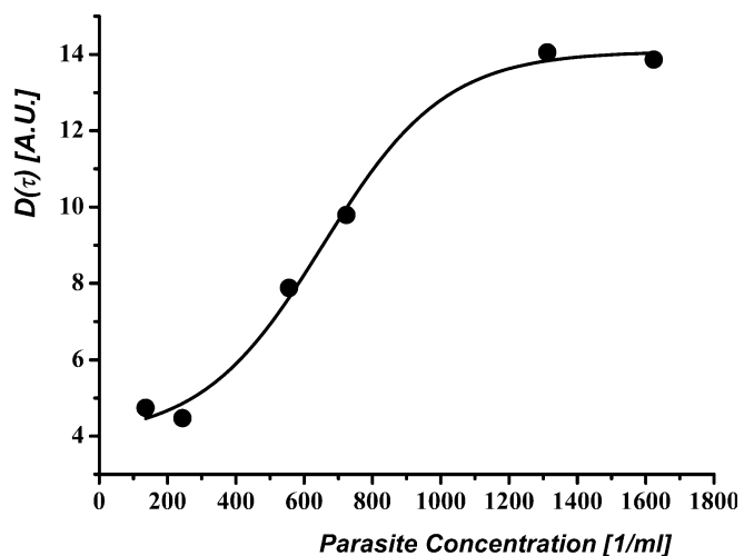
Fig. 3 Representation of the difference function, D(\tau) , as a function of the L3 concentration. A clear sigmoidal plot ( R^2=0.995 ) can be observed showing an approximate linear behavior for concentrations between 400 and 1000 \text{mL}^{-1}
