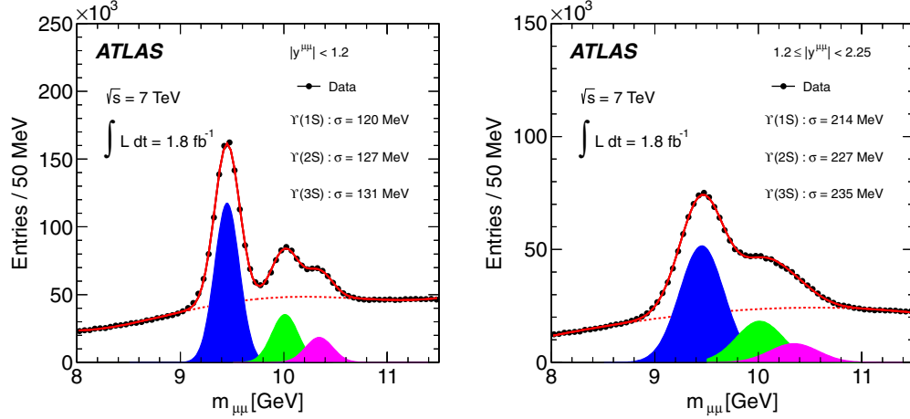
FIG. 1 (color online). The dimuon invariant mass spectrum for events used in this analysis. Separate spectra are shown for those events with the dimuon candidate (left) in the central region of the detector ( |y^{\mu\mu}| < 1.2 ) and (right) in the forward region ( 1.2 \leq |y^{\mu\mu}| < 2.25 ). Overlaid are individual shapes of the fitted Y(nS) signals (shaded regions), background-only fit (dashed curve), and the total signal plus background shape (solid curve). The background shape is modeled here by a fourth-order polynomial and the signal peaks each modeled by a single Gaussian. Also quoted are the fitted mass resolutions of each of the three signal peaks, determined from the fit with a common resolution parameter scaling with invariant mass.
