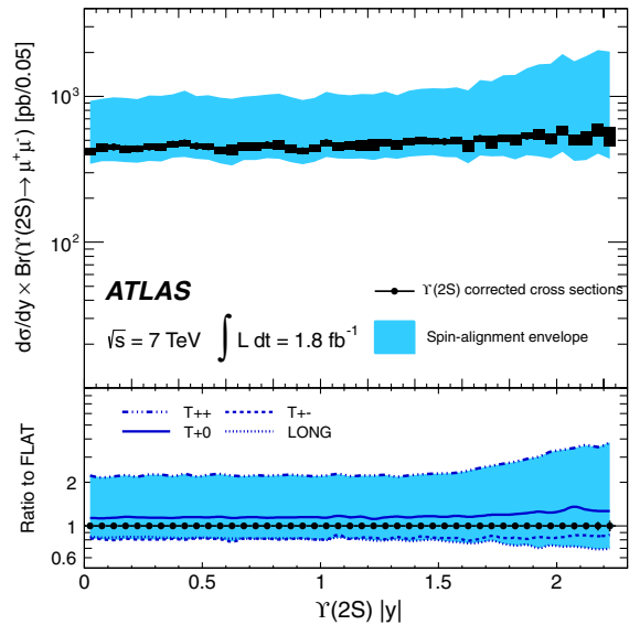
FIG. 16 (color online). As for Fig. 15, but for Y(2S) production.
