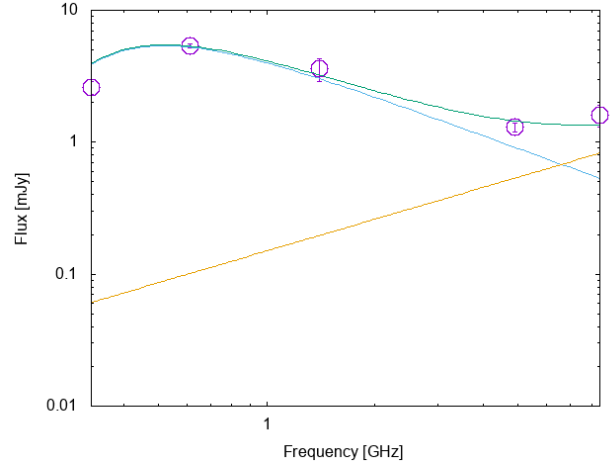
Figure 19. Measured spectrum of Cyg OB2-335 (magenta symbols); in green, the best fit adding thermal emission as 0.14 \nu^{0.7} (orange) plus non-thermal emission affected by FFA as 4.5 \nu^{-0.95} \exp(-0.13\nu^{-2.1}) (cyan).
