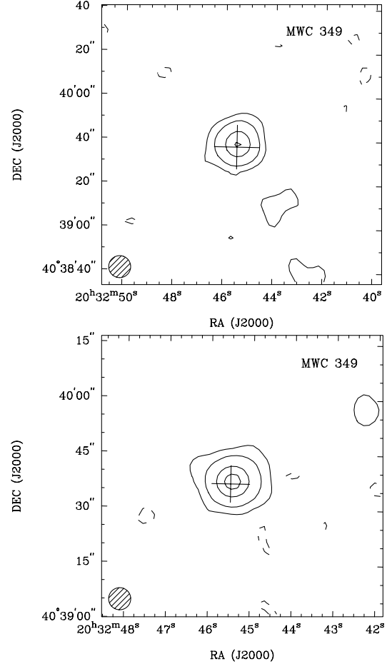
Figure 13. GMRT images of the system MWC 349. Top panel: at 325 MHz; contour levels of -0.7 , 0.9 ( =3\sigma ), 3 , 10 , and 17 \text{mJy beam}^{-1} . Bottom panel: at 610 MHz; contour levels of -0.3 , 0.3 ( =3\sigma ), 2 , 10 and 20 \text{mJy beam}^{-1} . Hatched, the synthesized beam. Cross hair: optical position of the system (Zacharias et al., 2012).
