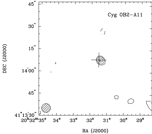
Figure 7. GMRT image of the star Cyg OB2-A11 at 610 MHz. The contour levels are -0.18 , 0.23 ( =3\sigma ), 0.3 , 0.4 and 0.45 mJy beam ^{-1} . Hatched, the synthesized beam. Cross hair: optical position of the system (see Table 2).
