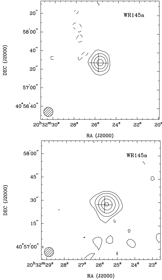
Figure 3. GMRT images of the system WR145a. Top panel: at 325 MHz; contour levels of -0.8 , 0.8 ( =3\sigma ), 4, 10 and 20 \text{mJy beam}^{-1} . Bottom panel: at 610 MHz; contour levels of -0.3 , 0.3 ( =2\sigma ), 2, 10, 30 and 60 \text{mJy beam}^{-1} . Hatched, the synthesized beam. Cross hair: optical position of the system (see Table 1).
