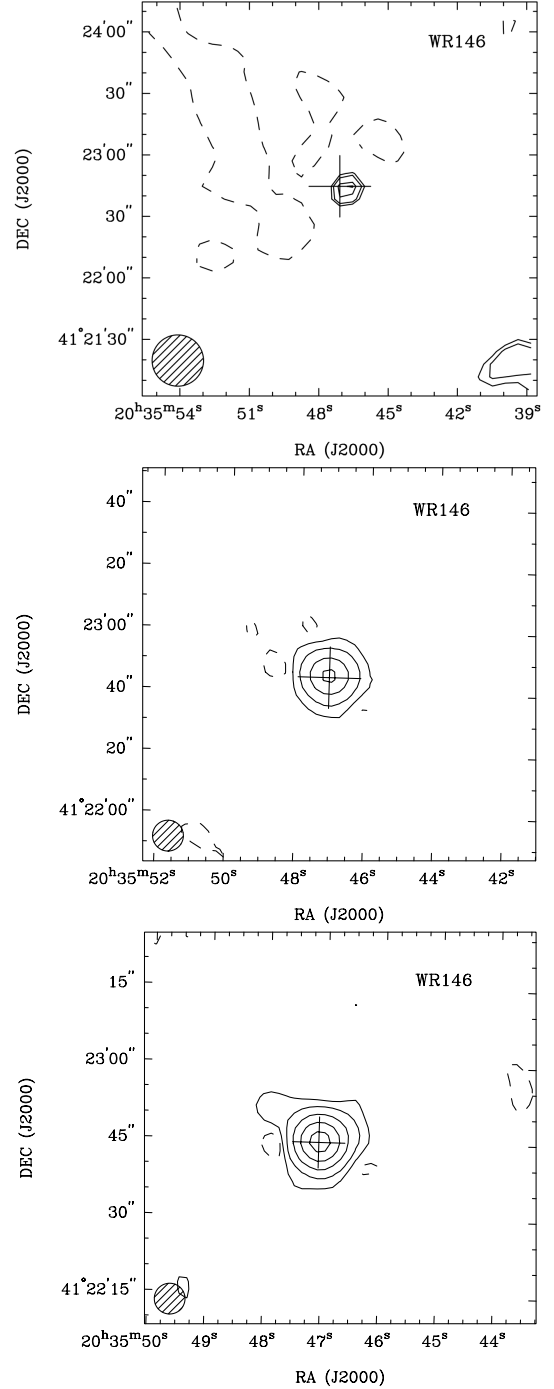
Figure 4. GMRT images of the system WR146. Top panel: at 150 MHz; contour levels of -18 , 18 ( =2\sigma ), 21, 27 and 30 \text{mJy beam}^{-1} . Central panel: at 325 MHz; contour levels of -1.5 , 1.5 ( =3\sigma ), 10, 40 and 90 \text{mJy beam}^{-1} . Bottom panel: contour levels of -0.75 , 0.75 ( =3\sigma ), 4, 15 and 40 \text{mJy beam}^{-1} . Hatched, the synthesized beam. Cross hair: optical position of the system (see Table 1).
