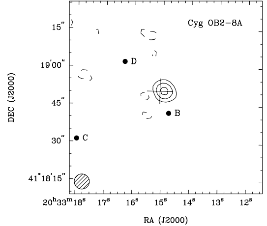
Figure 9. GMRT image of the system Cyg OB2-8A at 610 MHz. The contour levels are -0.35 , 0.30 ( =3\sigma ), 1 , 2 and 3 mJy beam ^{-1} . Hatched, the synthesized beam. The cross hair represents the optical position of the 8A system (see Table 2), and the filled circles, those of Cyg OB2-8B, -8C, and -8D stars (see Table 6).
