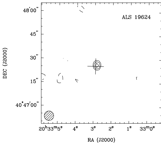
Figure 8. GMRT image of the star ALS 19624 at 610 MHz. The contour levels are -0.25 , 0.25 ( =3\sigma ), 0.35 and 0.46 mJy beam ^{-1} . Hatched, the synthesized beam. Cross hair: optical position of the system (see Table 2).
