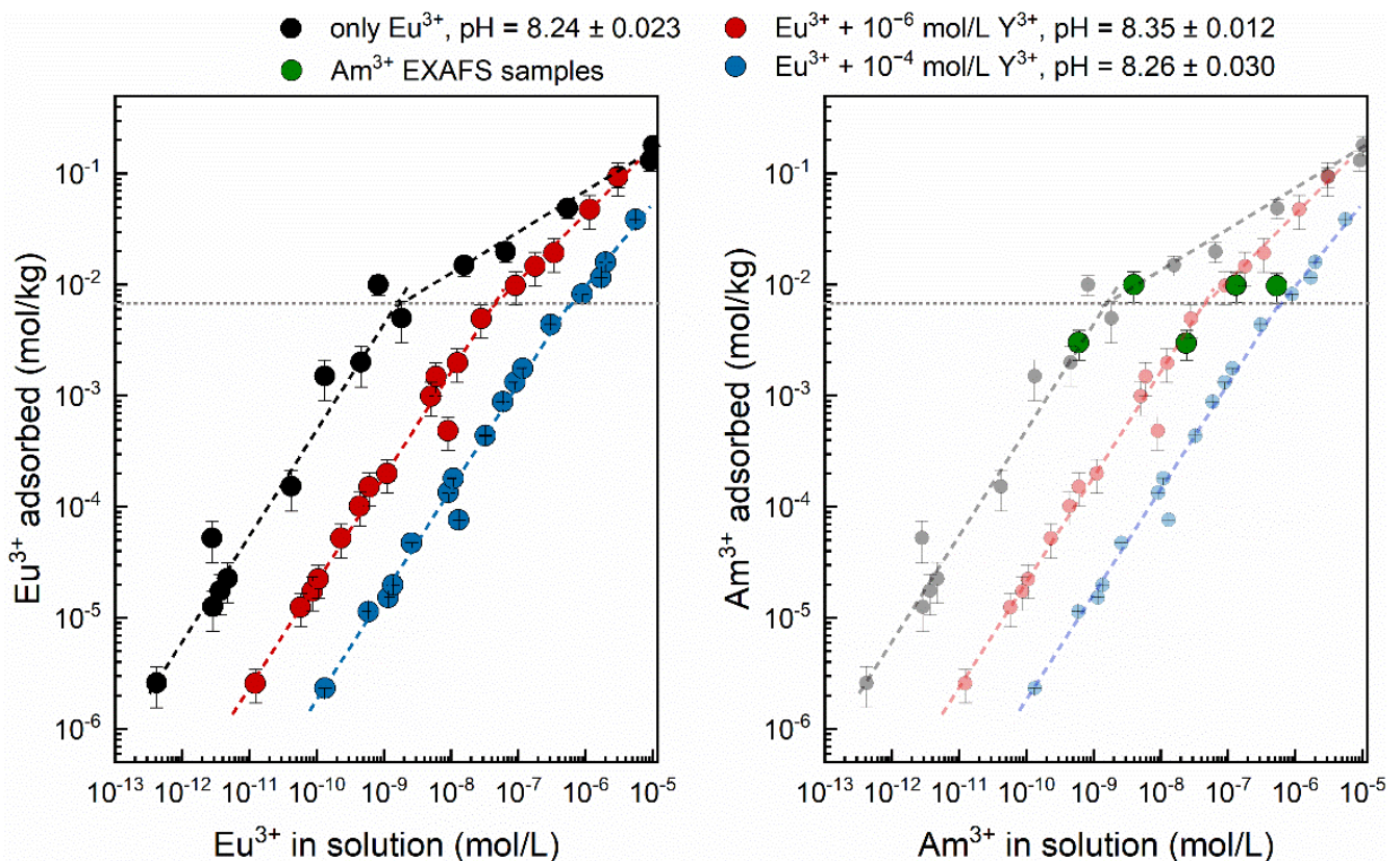
Figure 3. (Left): isotherm results for Eu^{3+} adsorption on 0.5 g/L corundum in the absence (black symbols) and presence of 10^{-6} mol/L (red symbols) and 10^{-4} mol/L Y^{3+} (blue symbols). The gray horizontal line indicates where the slope of the isotherm changes from one (1) to <1 . The error given for the pH values is the standard deviation ( 1\sigma ) of all sample pH values in one isotherm experiment. (Right): EXAFS samples (green symbols) containing Am^{3+} or Am^{3+} + Y^{3+} on 2.0 g/L corundum, displayed together with the Eu^{3+} isotherms (washed out symbols). For the pH values of these samples, the reader is referred to in Table 1.
