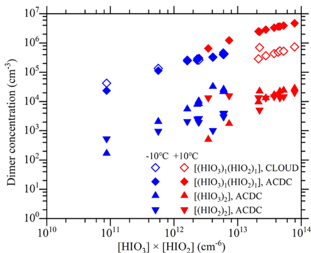
Figure 7. Measured (CLOUD) and simulated (ACDC) dimer concentrations ( [(\text{HIO}_3)_1(\text{HIO}_2)_1] , [(\text{HIO}_3)_2] , and [(\text{HIO}_2)_2] ) versus [\text{HIO}_3] \times [\text{HIO}_2] ( \text{cm}^{-6} ) at +10^\circ\text{C} (red symbols) and -10^\circ\text{C} (blue symbols). The hollow diamonds show [(\text{HIO}_3)_1(\text{HIO}_2)_1] measured by CLOUD. The filled symbols show dimer concentrations from ACDC simulations based on our quantum chemical calculations: filled diamonds for [(\text{HIO}_3)_1(\text{HIO}_2)_1] , filled pyramids for [(\text{HIO}_3)_2] , and filled inverted pyramids for [(\text{HIO}_2)_2] .
