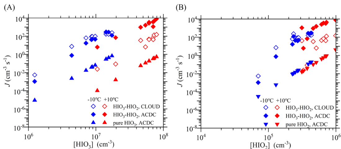
Figure 6. Measured (CLOUD) and simulated (ACDC) neutral cluster formation rates J versus (A) [\text{HIO}_3] and (B) [\text{HIO}_2] at +10^\circ\text{C} (red symbols) and -10^\circ\text{C} (blue symbols). The hollow diamonds show iodine oxoacid cluster formation rates from CLOUD. The filled symbols show cluster formation rates from ACDC simulations based on our quantum chemical calculations: iodine oxoacid clusters (filled diamonds), pure \text{HIO}_3 clusters (filled pyramids), and pure \text{HIO}_2 clusters (filled inverted pyramids).
