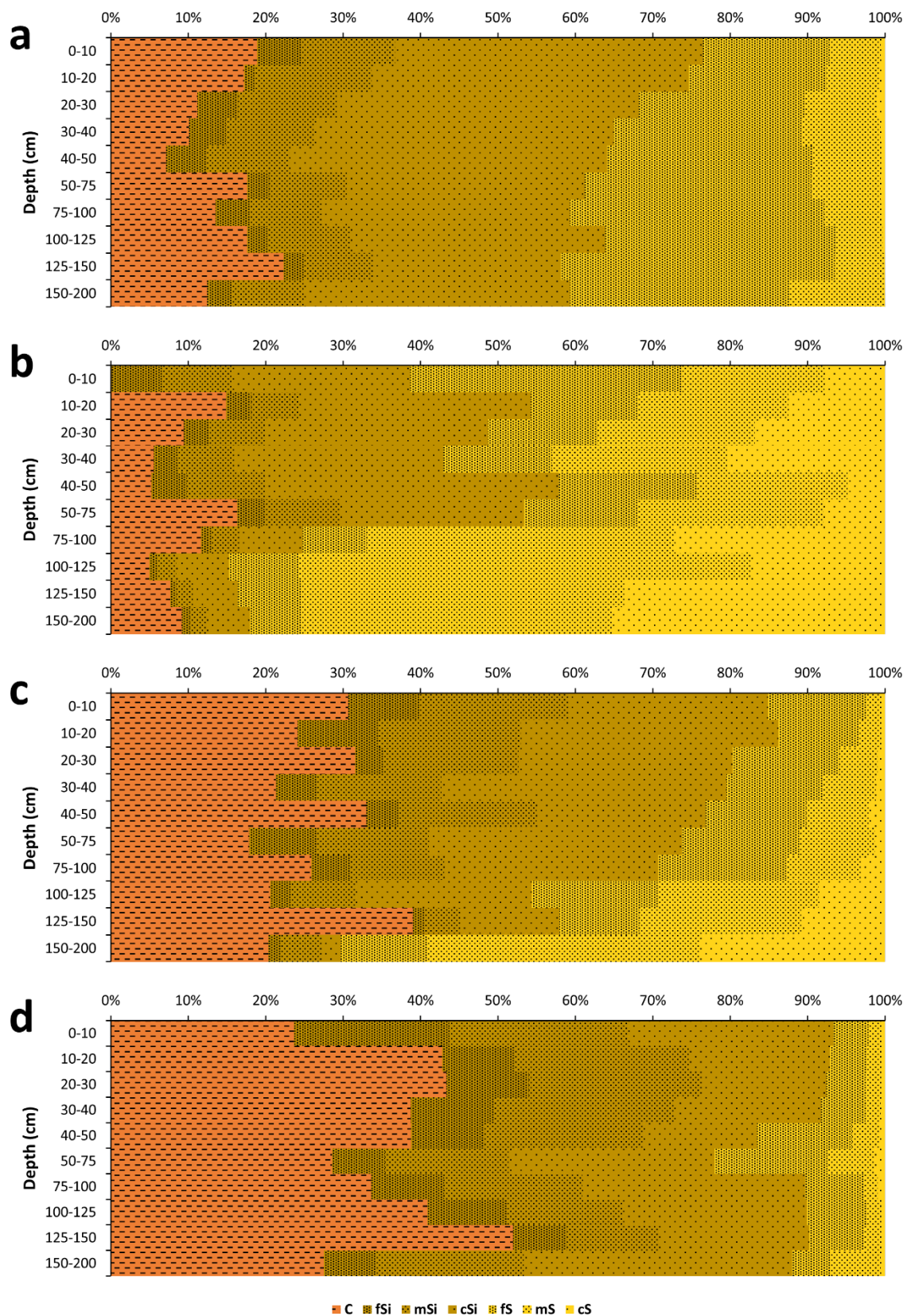
Figure S3: Grain size distribution for soil profiles of site STD. a: Profile STD-1, b: Profile STD-2, c: Profile STD-3, d: Profile STD-4.
