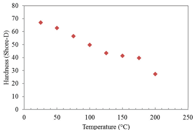
FIGURE 4. Temperature effect on hardness
