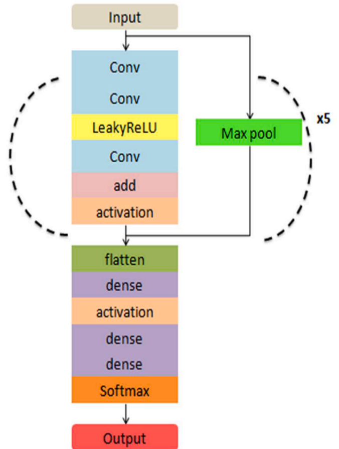
Fig. 11. Architecture of the proposed 1D-CNN model.
