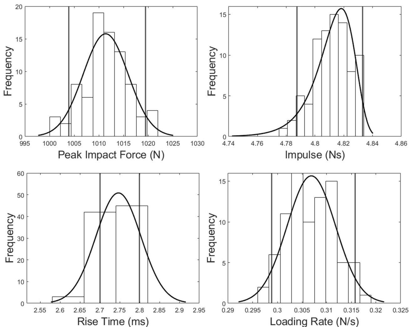
Fig. 2 Histograms with distribution fit for peak impact force, impulse, rise time and loading rate at 6.04 \text{ m s}^{-1}
