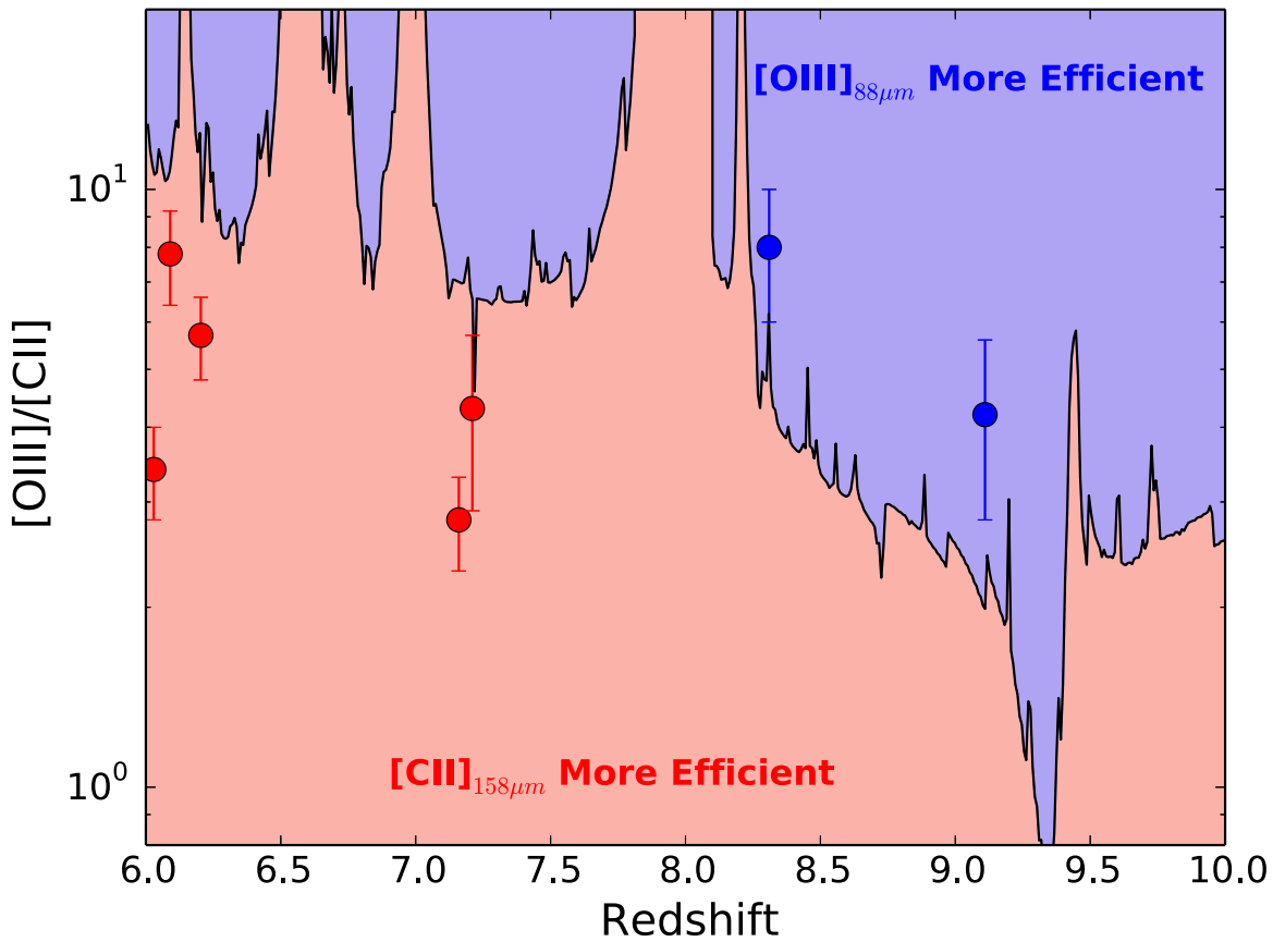
Figure 6. The break-even [\text{O III}]_{88\ \mu\text{m}}/[\text{C II}]_{158\ \mu\text{m}} luminosity ratio where [\text{C II}]_{158\ \mu\text{m}} and [\text{O III}]_{88\ \mu\text{m}} scans are equally efficient to execute (Section 3.1). The plotted red and blue circles show the measured [\text{O III}]_{88\ \mu\text{m}}/[\text{C II}]_{158\ \mu\text{m}} luminosity ratios for specific high-redshift sources (Hashimoto et al. 2019; Bakx et al. 2020; Carniani et al. 2020; Harikane et al. 2020) featuring \geq 5\sigma line detections and where the emission is largely cospatial (but see Carniani et al. 2017). For luminosity ratios in the red regions, [\text{C II}]_{158\ \mu\text{m}} scans are more efficient, while for luminosity ratios in the blue regions, [\text{O III}]_{88\ \mu\text{m}} scans are more efficient. The break-even ratios are computed based on the integration times required to detect [\text{C II}]_{158\ \mu\text{m}} and [\text{O III}]_{88\ \mu\text{m}} lines at a given redshift and rely on the atmospheric transmission at a given frequency using the equations in the ALMA Technical Handbook (Cortes et al. 2020). Use of the [\text{C II}]_{158\ \mu\text{m}} line for spectral scans seems to be more efficient for galaxies at z = 6.5\text{--}8.2 , while use of the [\text{O III}]_{88\ \mu\text{m}} line for spectral scans seems to be more efficient for galaxies at z > 8.5 .
