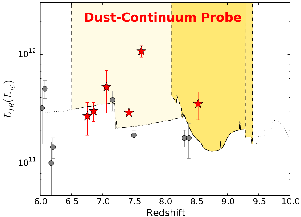
Figure 9. The 3.3\sigma limiting IR luminosities probed by the REBELS scans for [\text{C II}]_{158 \mu\text{m}} and [\text{O III}]_{88 \mu\text{m}} in 40 very bright reionization-era galaxies (light yellow and gold shaded regions, respectively). The red stars show the IR luminosities of six z = 7 – 8 galaxies from the REBELS pilot programs (Schouws et al. 2022a; Smit et al. 2018) while the gray circles show the IR luminosities inferred for various dust-detected galaxies in the literature. REBELS will detect sources in the dust continuum if their IR luminosities are greater than 3 \times 10^{11} L_{\odot} to z \sim 7.2 and down to 2 \times 10^{11} L_{\odot} at z = 7.2 – 9.4 (equivalent to obscured SFRs of 36 M_{\odot} \text{ yr}^{-1} and 24 M_{\odot} \text{ yr}^{-1} , respectively). Extrapolating our pilot results, the REBELS program is projected to increase the number of dust detections by 3 – 4\times at z > 6.5 , and will allow us to test whether large dust reservoirs are common (as suggested by our detections and also the Watson et al. (2015) and Laporte et al. (2017) sources at z \sim 7.5 and z = 8.38 , respectively) or whether there is a rapid decline in IR bright galaxies at z > 7.5 .
