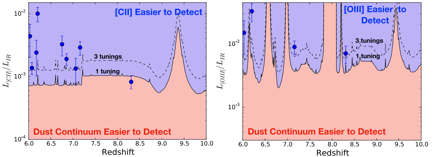
Figure 8. The break-even [\text{C II}]_{158 \mu\text{m}}/\text{IR} and [\text{O III}]_{88 \mu\text{m}}/\text{IR} luminosity ratio (left and right panels, respectively) for both detection ( 5\sigma ) of the [\text{C II}]_{158 \mu\text{m}} and [\text{O III}]_{88 \mu\text{m}} lines and detection ( 3.3\sigma ) of the dust continuum shown as a function of redshift. Also shown on this diagram are z \sim 6 – 10 sources from the REBELS pilot programs (Smit et al. 2018; Schouws et al. 2022a, 2022b) and the literature (Hashimoto et al. 2019; Tamura et al. 2019; Bakx et al. 2020; Harikane et al. 2020). The dashed lines show the break-even ratios assuming three separate tunings for a spectral scan. The use of >3 tunings would shift the break-even ratio to even higher values. For the typical source, one can clearly consider up to six tunings per source before the line sensitivity of ALMA becomes the limiting factor in probing both line and continuum emission. This fits very well with the spectral scan strategy employed in REBELS, where the aim is to probe both lines and the dust continuum.
