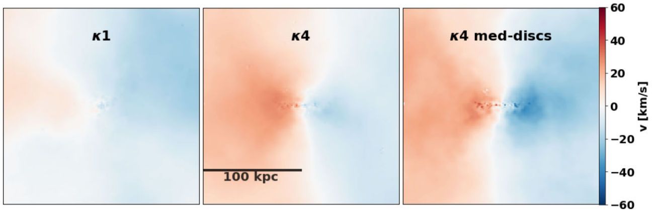
Figure 12. Projected line-of-sight velocity of gas with T > 10^{5.3} K for the \kappa 1 , \kappa 4 , and \kappa 4 -med-discs samples, which are rotated to have their velocities aligned. The med-discs sample has the highest hot gas rotation aligned with the stellar disc. The low level of preferred rotation in the \kappa 1 sample probably arises because these galaxies were also rotated based on their stellar velocities.
