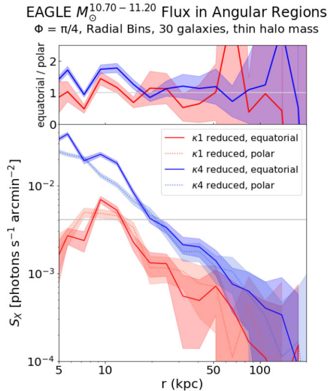
Figure 8. Stacks of 30 galaxies within a thin halo mass range, M_{200} = 10^{12.49-12.71} M_{\odot} , to isolate the effect of morphology independent of halo mass dependence. The \kappa 4 sample shows a similar split between the equatorial and polar regions as Fig. 6, while the \kappa 1 sample is dimmer with larger errors.
