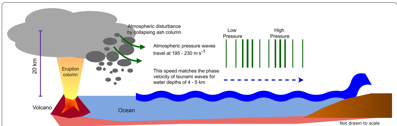
Fig. 5 Generation of volcanic-meteotsunamis (VMTs). Collapsing eruption column produces atmospheric pressure waves. If the lateral speed of the atmospheric waves matches the tsunami waves, water resonance occurs, amplifying the VMTs. Adapted from original by Lowe and De Lange (2000)
