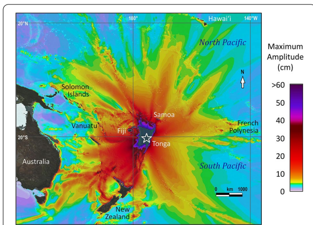
Fig. 4 Modelled maximum tsunami amplitude following the eruption of HTHH volcano on 15 January 2022. The location of the volcano in Tonga is indicated by the white star. The propagation does not include any tsunami component induced by atmospheric shockwaves. Base image courtesy of the NOAA Center for Tsunami Research (NOAA 2022)
