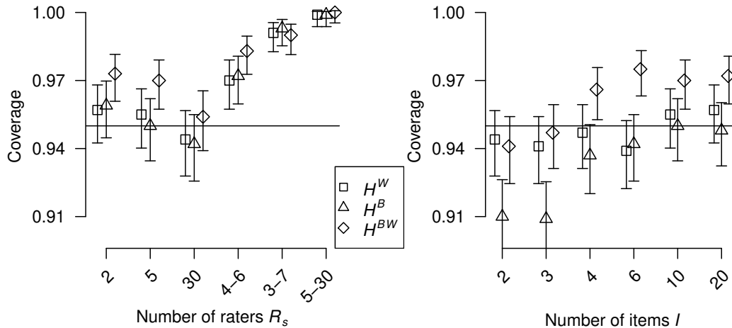
Figure 4.2: Coverage plots for the two-level scalability for different number of raters and items, respectively. Error bars represent the 95% Agresti-Coull confidence interval.
