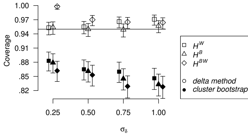
Figure 4.1: Plot of the coverage of the 95% confidence interval of the two-level scalability coefficients, for different levels of rater effect \sigma_\delta and the two standard error estimation methods. Error bars represent the 95% Agresti-Coull confidence interval.
