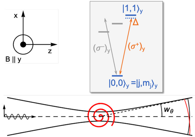
Figure 2: Optical analog of the Magnus effect. A linearly polarized ( \mathbf{E} \parallel x ), focused laser induces a circular dipole ( xz plane) on a j = 0 \rightarrow j' = 1 ( \Delta m_j = 1 ) transition, with a magnetic field \mathbf{B} \parallel y setting the quantization axis. The spiral wave scattered by the circular dipole interferes with the incident wave. Due to the relative tilt between the wavefronts (exaggerated for clarity), interference may shift the optical power to one side of the beam, thus deflecting the beam in the xz plane. The corresponding reaction force on the atom, can shift the equilibrium trapping position in an optical tweezer away from the optical axis by an amount \tilde{\lambda} = \lambda/2\pi , see text and Figure 4.
