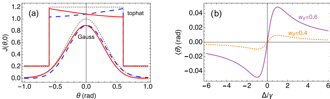
Figure 3: Beam deflection or Magnus effect analogy.
