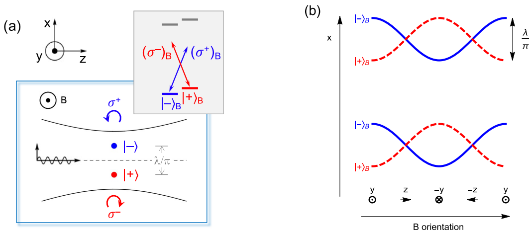
Figure 4: Spin dependent displacement and motion in optical tweezers.
