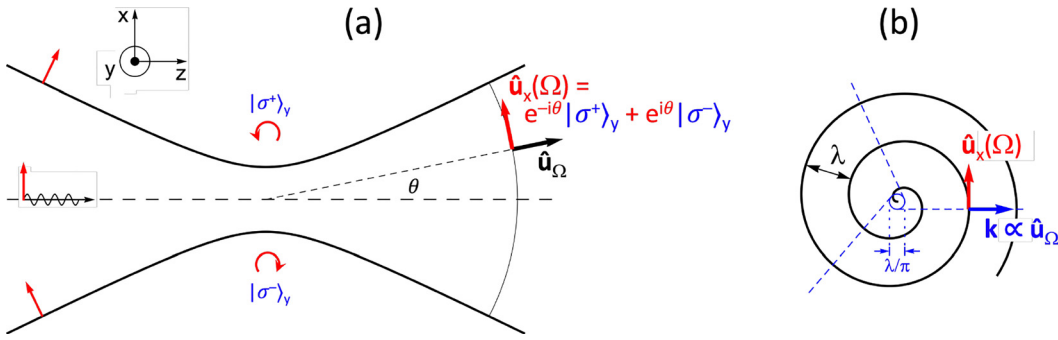
Figure 1: Examples of nonparaxial light fields with ‘intertwined’ SAM and OAM.
