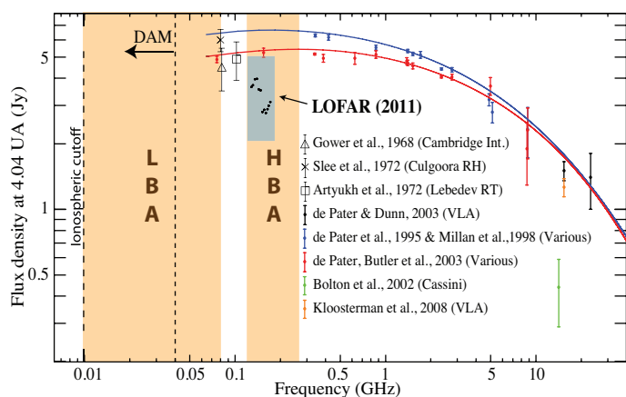
Fig. 8. Measurements of Jupiter’s synchrotron spectrum at meter to centimeter wavelengths, scaled to the distance of 4.04 AU. The majority of the measurements was obtained with the VLA between 1991 and 2004 (de Pater et al. 1995; Millan et al. 1998; de Pater & Dunn 2003; de Pater & Butler 2003; de Pater et al. 2003; Kloosterman et al. 2008), some of which were after the impact of Comet Shoemaker-Levy 9 in 1994. The blue and red curves were fitted by de Pater et al. (2003) to the series of measurements taken respectively in 1994 and 1998. LOFAR measurements of the present study are the black dots in the HBA range, and their uncertainty is figured by the grey box. Previous measurements below \sim 300 MHz are unresolved. Decameter emission (DAM – not shown) dominates the spectral range below 40 MHz (see Fig. 1b).
