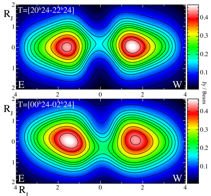
Fig. 9. Simulated synchrotron images derived from Salammbô-3D (see text) of the emission averaged over the full band at two periods: i) [20h24–22h24] UT (CML=[ 9^\circ – 82^\circ ]), min/max=[ 8 \times 10^{-3} , 0.475] Jy/beam and ii) [00h24–02h24] UT (CML=[ 154^\circ – 227^\circ ]), min/max=[ 8 \times 10^{-3} , 0.467] Jy/beam. The synchrotron maps were computed with the same observation parameters as in Fig. 5b) and d). Contours highlight the brightness by steps of 10% of the maximum.
