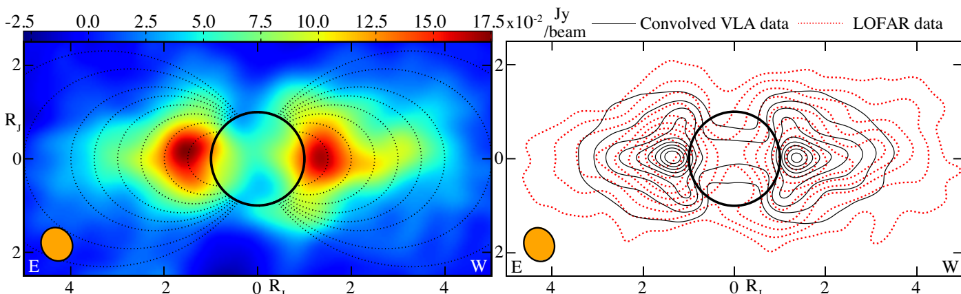
Fig. 6. Best LOFAR high resolution image to date of Jupiter’s radiation belts, integrated over the entire 23 MHz band of observation distributed from 127 and 172 MHz, and a 7 hour interval from \sim 19:00 to \sim 02:00 UT. The same image is displayed in both panels with color scale (left) and contours (right). The frequency-averaged clean beam size and shape ( \sim 18'' \times 16'' ) is displayed at the bottom left of each panel. Pixel size is 1'' \times 1'' . R.m.s. noise is 4.7 mJy/beam and the SNR (maximum peak flux divided by standard deviation) is 37. The SNR is approximately 14 at the 30 % flux level (corresponding to the extremity of the emission). Dipolar field lines with apex at 1.5, 2, 2.5, 3, 3.5, 4 & 5 R_J are superimposed on the left panel. Contours superimposed on the right panel are derived from a rotation-averaged VLA image (obtained from Santos-Costa et al. 2009, in C band) which has been convolved down to match the LOFAR observation angular resolution. Each set of contours represents relative intensity levels by steps of 10 % of the maximum radiation peak: in the convolved VLA image (black line) and in the LOFAR image (red dotted line).
