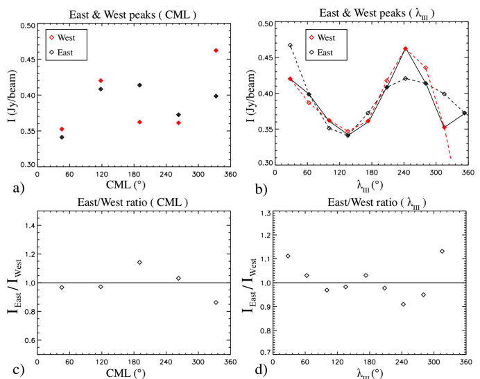
Fig. 12. a) east and west peak intensities in each frequency-averaged image, as a function of the CML at the middle of the 2 hour interval corresponding to each image. b) east and west peak intensities – as a proxy of the peak emissivity – as a function of \lambda_{III} , derived from a) following the sketch of Fig. 11. Measured values are filled diamonds connected by the solid line. Open diamonds are interpolated from a spline adjustment of east and west measurements separately. Dashed lines are the two resulting independent determinations of the peak emissivity profiles versus \lambda_{III} . c,d) east-to-west peak intensity ratios deduced from panels a) and b).
