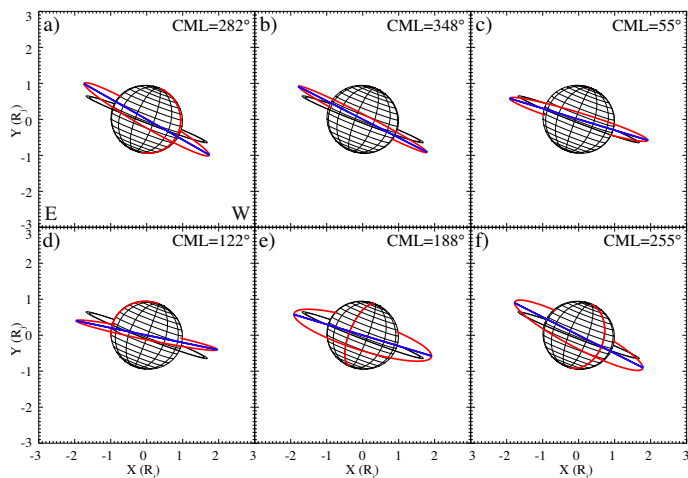
Fig. 3. Wobbling of the Jovian magnetic equator (red circle) on the plane of the sky during one planetary rotation. The rings (in black) lie in the rotational equator. The blue line represents the main axis of the projection on the sky of the magnetic equator, which should also be the main axis of the radiation belts image as a function of time or longitude. Observer’s longitude (CML) is indicated on each panel as well as the reference meridian (in red).
