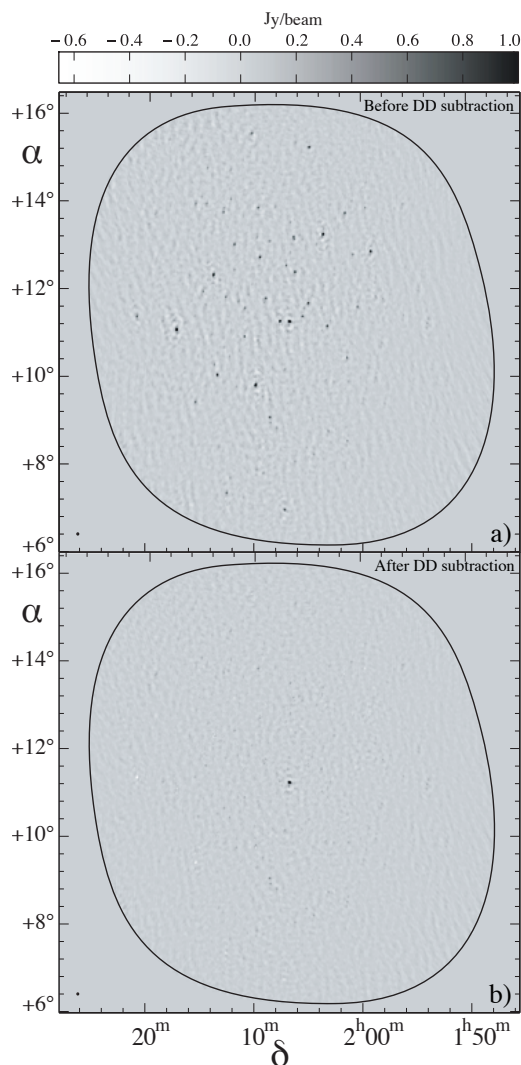
Fig. 4. Wide-field ( 8^\circ \times 8^\circ ) image of the target field before a) and after b) DD subtraction. The central frequency is 143 MHz and the bandwidth is 1.9 MHz (SB 40–49). The image is 2100 \times 2100 pixels of 18'' , baseline length was restricted to \leq 10 k \lambda to ensure a good sampling of the PSF. A natural weighting was used and deconvolution with AWimager (implementing A-projection and W-projection) with 10 000 iterations and a CLEAN gain of 0.1. The angular resolution is \sim 2.5' . The r.m.s. and the SNR are respectively 37 mJy/Beam and 71 in the non-peeled image (a) and \sim 27 mJy/Beam and 98 in the peeled image (b). Sixty background sources have been automatically identified and subtracted in panel a) to obtain the image of panel b). Jupiter lies at the center of the field. The beam size and shape are displayed at the bottom left of each panel.
