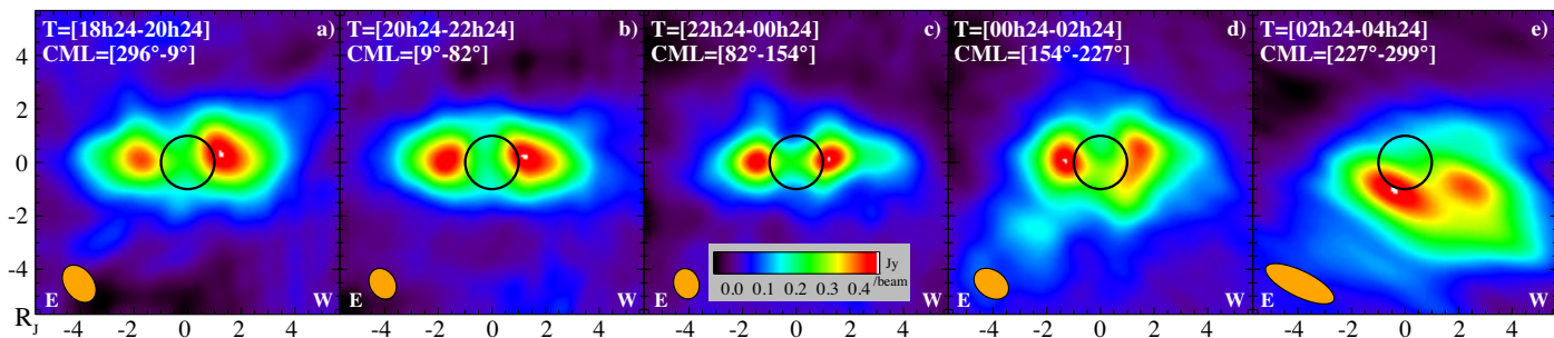
Fig. 5. Zoomed images of Jupiter’s radiation belts obtained after motion corrections in the (u,v) plane and DD subtraction, in a \sim 10' \times 10' field, integrated over the whole bandwidth for the same time intervals as Fig. 2. The spatial scale is given in Jovian radii at Jupiter ( 1 R_J = 71492 km, corresponding to \sim 49'' in the sky at observation epoch). Imaging was performed with baselines \leq 15 k \lambda , giving a theoretical angular resolution of 14'' and an effective angular resolution ranging from 20'' to 78'' over the 10 hours. Pixel size is 2'' \times 2'' . In the five successive images a) to e), the residual noise level is 14.9, 10.5, 12.3, 15.9 and 21.2 mJy/beam, and the peak SNR ratio is respectively 31.0, 33.6, 34.1, 26.0 and 17.6. The last image is more distorted because of the low source elevation during that observing interval.
