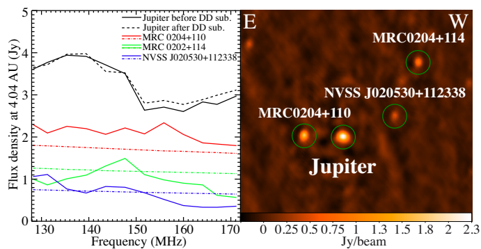
Fig. 7. a) Wide-field unresolved image of Jupiter and its vicinity (zoom in a region of \sim 1.2^\circ \times 1.2^\circ ) before source subtraction. The 3 bright nearby radio sources have the following flux density S at 73.8 MHz and spectral index \alpha (following the convention S_\nu \propto \nu^\alpha ): S=2.24 \pm 0.23 Jy and \alpha = -1.0 for MRC 0204+110 ; S=1.00 \pm 0.12 Jy and \alpha = -0.9 for NVSS J020530+112338 ; S=1.94 \pm 0.17 Jy and \alpha = -0.9 for MRC 0202+114 (see NED database ned.ipac.caltech.edu). b) Measured spectra of these 3 radio sources at 12 frequencies between 127 and 172 MHz (solid color lines) compared with NED predictions (dash-dot color lines). The black lines show the total integrated flux density measured on the unresolved image of Jupiter before and after DD subtraction of surrounding radio sources at the same 12 frequencies. The difference between the two black lines is marginal.
