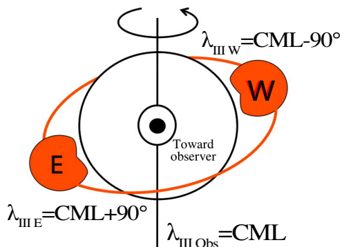
Fig. 11. Sketch of the relationship between observer's CML and System III longitude of the east and west sides of a synchrotron image of Jupiter.
