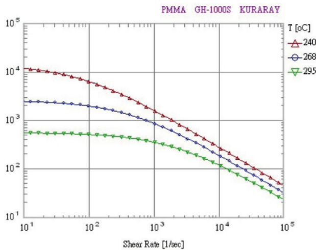
Fig. 7 KURARAY PMMA's shear viscosity curve
