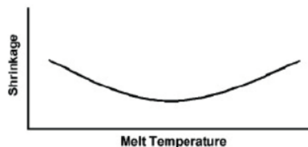
Fig. 12 Melt temperature and shrinkage curve [19]
