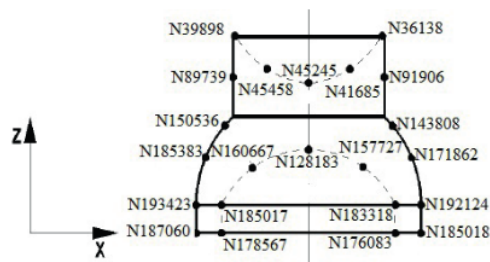
Fig. 17 Node setting in the molded part
