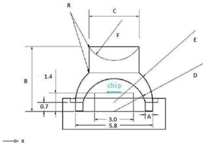
Fig. 3 Schematic of the new lens
