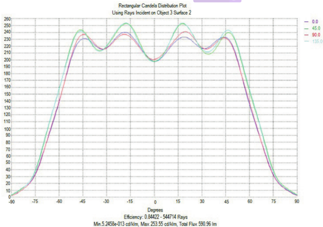
Fig. 18 Rectangular luminance distribution of the new lens
