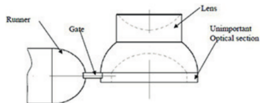
Fig. 5 Schematic drawing of gate, runner and cavity
