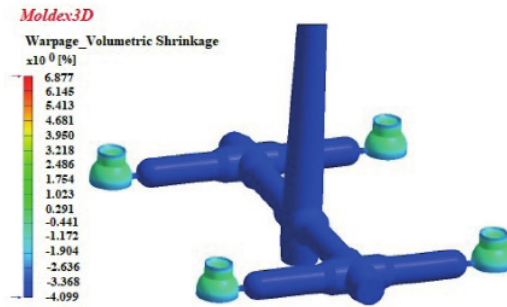
Fig. 15 Volumetric shrinkage value of the optimal molded part Article Error ETS
