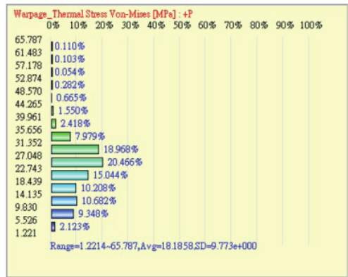
Fig. 16 Total thermal residual stress value of the optimal molded part
