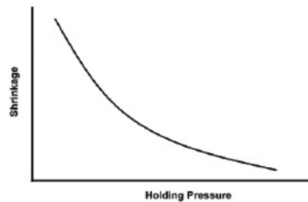
Fig. 10 The relationship between shrinkage and packing pressure [19]
