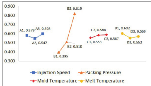
Fig. 13 Factors effect on Grey grade value
