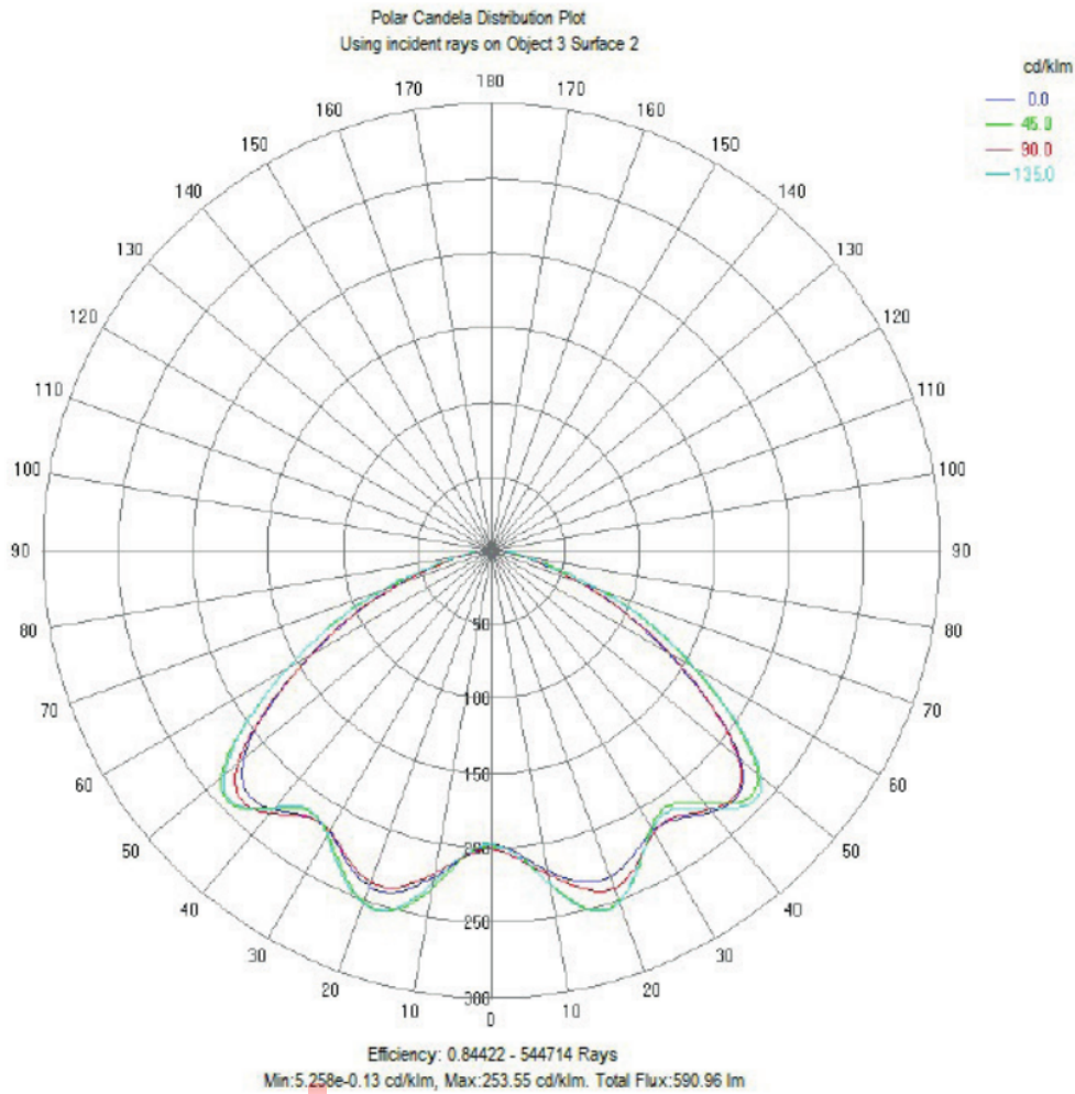
Fig. 19 Polar luminance distribution of the new lens
