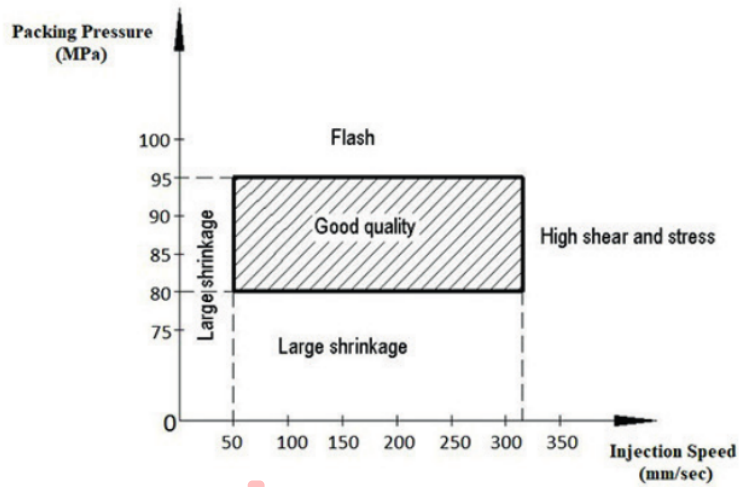
Fig. 8 The lens processing window
