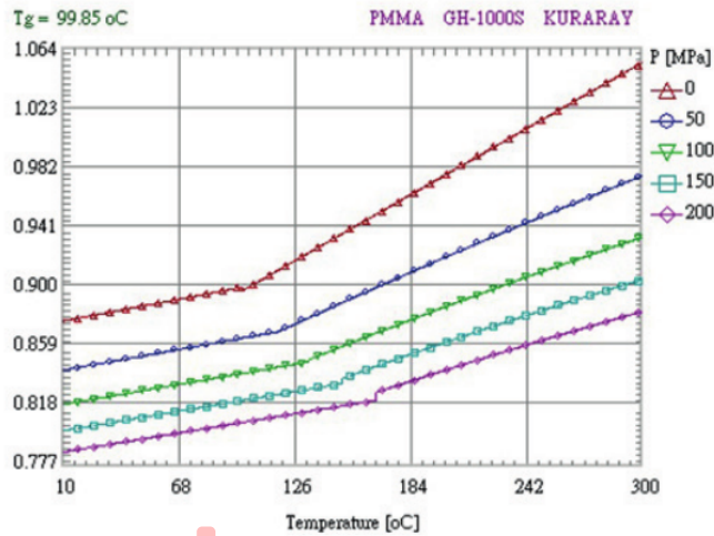
Fig. 6 KURARAY PMMA's PvT diagram
