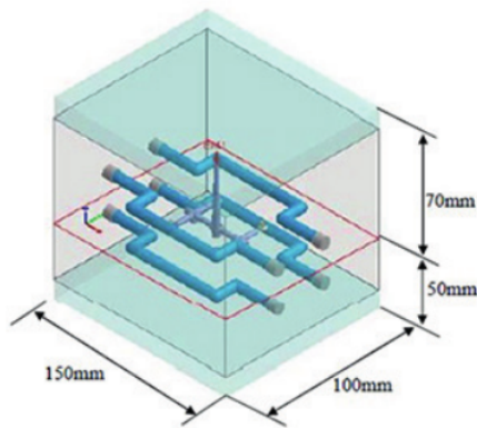
Fig. 4 Schematic picture of the mold system
