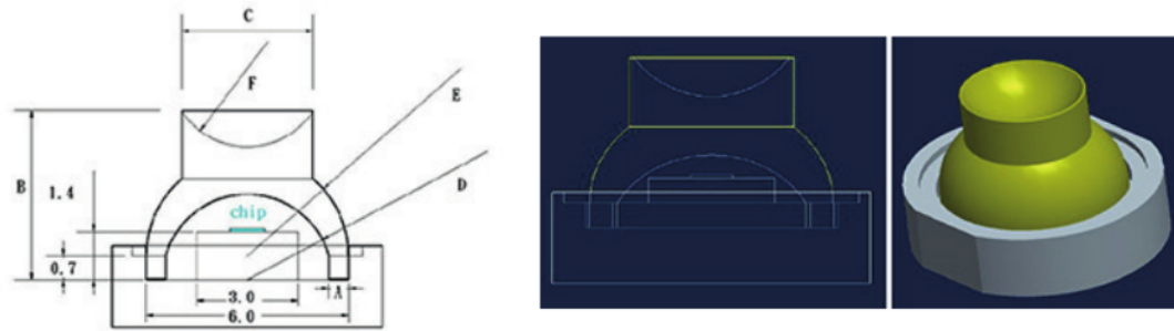
Fig. 1 Original Lens design and LED base
