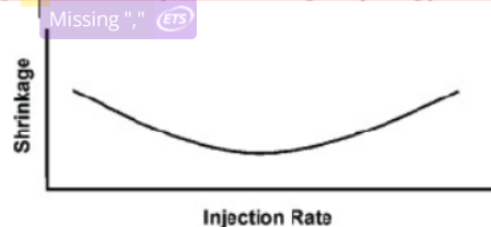
Fig. 11 The relationship between injection rate and shrinkage [19]
