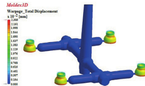
Fig. 14 Total displacement value of the optimal molded part
