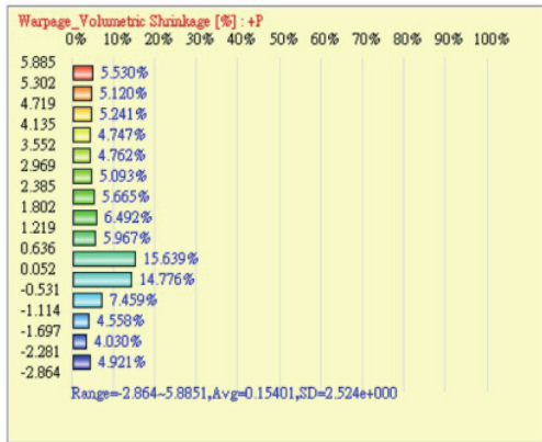
Fig. 15 Volumetric shrinkage value of the optimal molded part Article Error ETS
