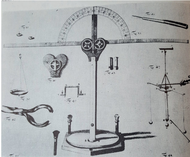
Fig. 11. Gralath–Kühn electrostatic scale with its equipment (Kühn 1747).
