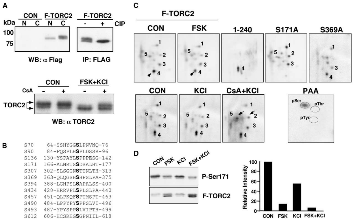
Figure 4. cAMP and Calcium Influx Promote Dephosphorylation of TORC2 at Ser171
