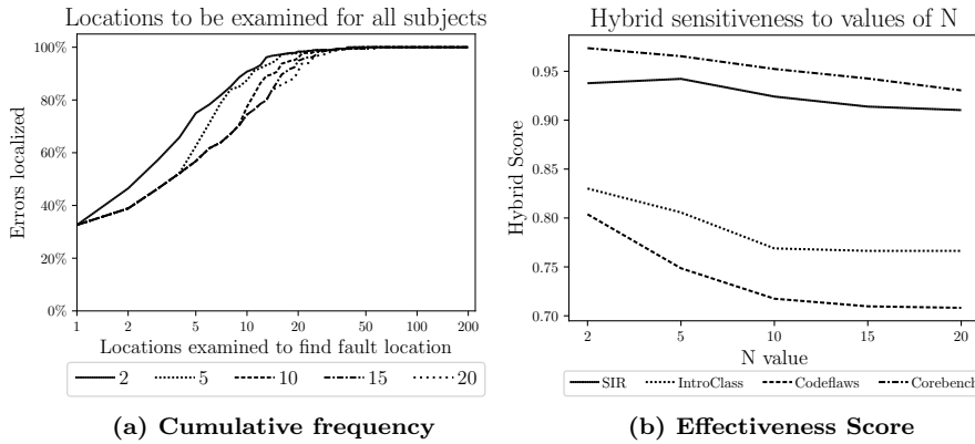
Fig. 9 Hybrid sensitiveness to different values of N \in \{2, 5, 10, 15, 20\} showing (a) the cumulative frequency of locations to be examined for all errors (left), and (b) the effectiveness score for each benchmark using the hybrid approach (right).
