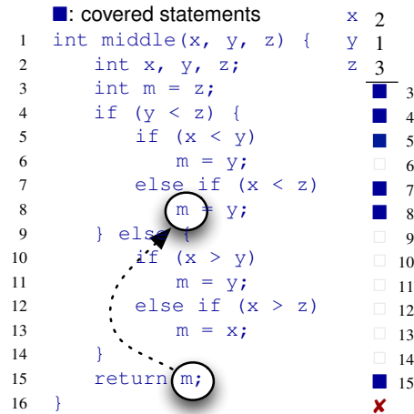
Fig. 2 Dynamic slicing illustrated (Jones and Harrold, 2005): The middle return value in Line 15 can stem from any of the assignments to m , but only those in Lines 3 and 8 are executed in the failing run. Following back the dynamic dependency immediately gets the programmer to Line 8, the faulty one.
