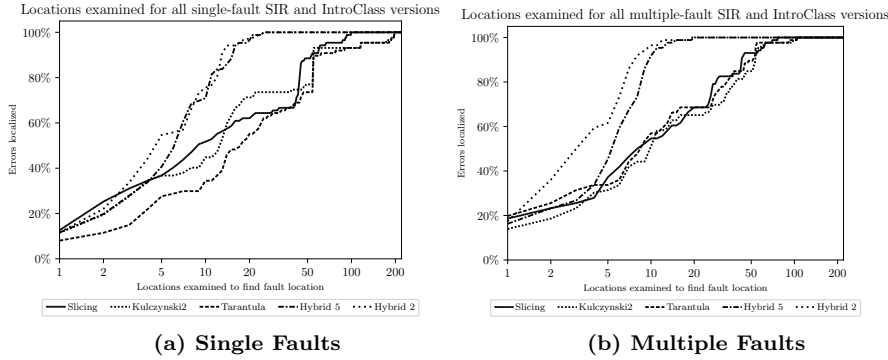
Fig. 11 Cumulative frequency of the locations to be examined for (a) single-fault and (b) multiple-fault versions of the SIR and IntroClass, using the hybrid approach, statistical debugging (Kulczynski2 and Tarantula) and dynamic slicing
