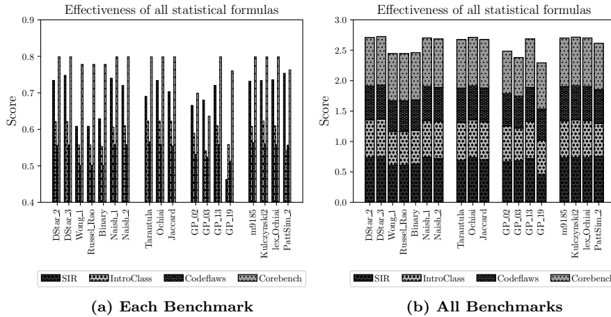
Fig. 5 Effectiveness of each SBFL formula on Single Faults; Results are grouped into bars for each family showing (a) the performance of each SBFL formula on each benchmark and (b) the cumulative results for all benchmarks using stacked bars
