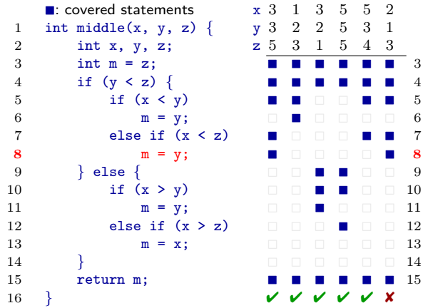
Fig. 1 Statistical debugging illustrated (Jones and Harrold, 2005): The middle function takes three values and returns that value which is greater than or equals the smallest and less than or equals the biggest value; however, on the input (2, 1, 3), it returns 1 rather than 2. Statistical debugging reports the faulty Line 8 (in bold red ) as the most suspicious one, since the correlation of its execution with failure is the strongest.
