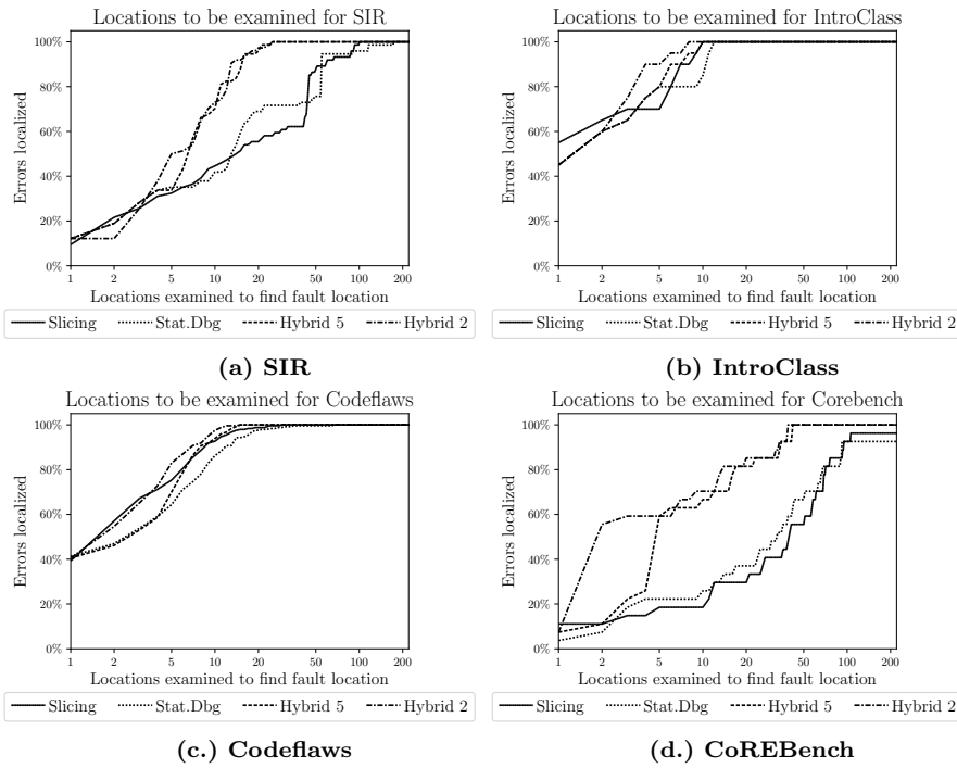
Fig. 8 Cumulative frequency of the locations to be examined, for dynamic slicing vs. statistical debugging vs. the hybrid approach (on single faults) in each benchmark
