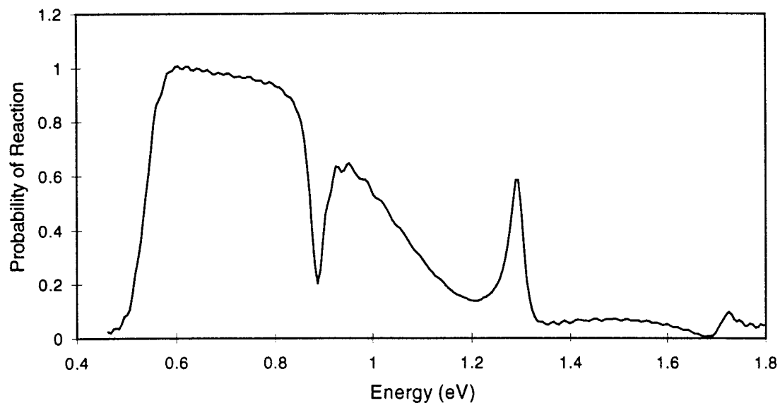
Figure 4.9 Probability of reaction calculated using the channel packet method with absorbing boundary conditions for H + H_2(v = 0) \rightarrow H_2(v' = 0) + H .
