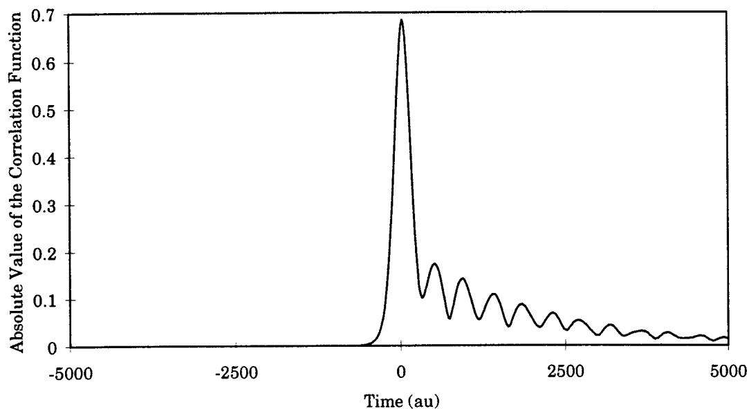
Figure 5.15 Absolute value of the correlation function for the two coupled Morse oscillator MLM mass configuration for the reaction A + BC(\nu = 0) \rightarrow AB(\nu' = 0) + C . In this calculation, the ABC are first constructed in Jacobi coordinates and then transformed to bond coordinates.
