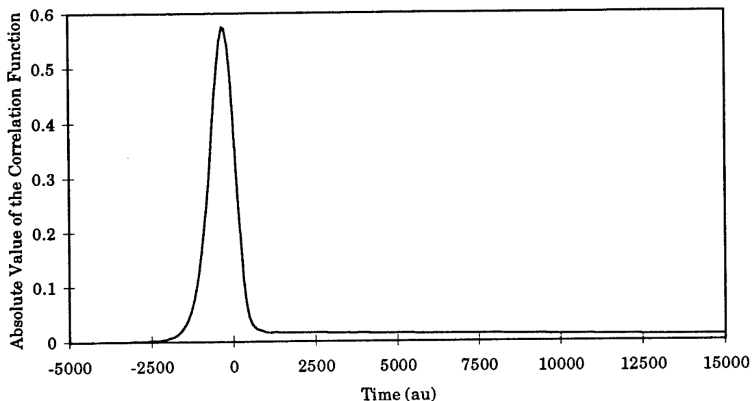
Figure 5.23 Absolute value of the correlation function for the two coupled Morse oscillator HLH mass configuration for the reaction A + BC (\nu = 0) \rightarrow AB (\nu' = 0) + C where absorbing boundary conditions were not used.
