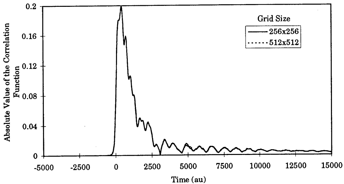
Figure 6.2 Absolute value of the correlation function for the two coupled Morse oscillator LHL mass configuration for the reaction A + BC(\nu = 0) \rightarrow AB(\nu' = 0) + C for two different grid sizes. For the larger grid size, the absorbing boundary conditions are placed further away from the interaction region.
