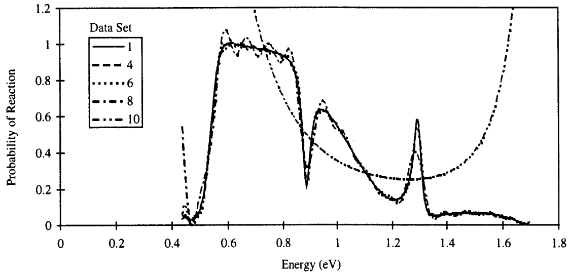
Figure 4.11 Convergence of the probability of reaction using the channel packet method with absorbing boundary conditions towards the correct answer for the reaction H + H_2(v = 0) \rightarrow H_2(v' = 0) + H .
