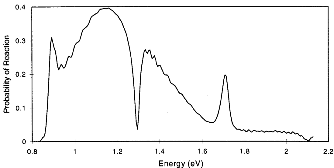
Figure 4.10 Probability of reaction calculated using the channel packet method with absorbing boundary conditions for H + H_2(v = 0) \rightarrow H_2(v' = 1) + H .
