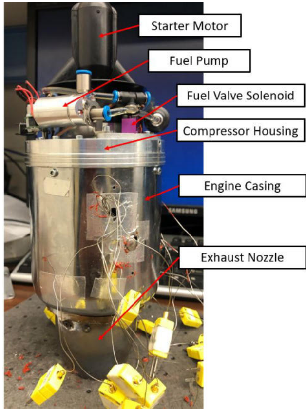
Figure 47. JetCat P160-RXi-B engine fully reassembled with instrumentation
