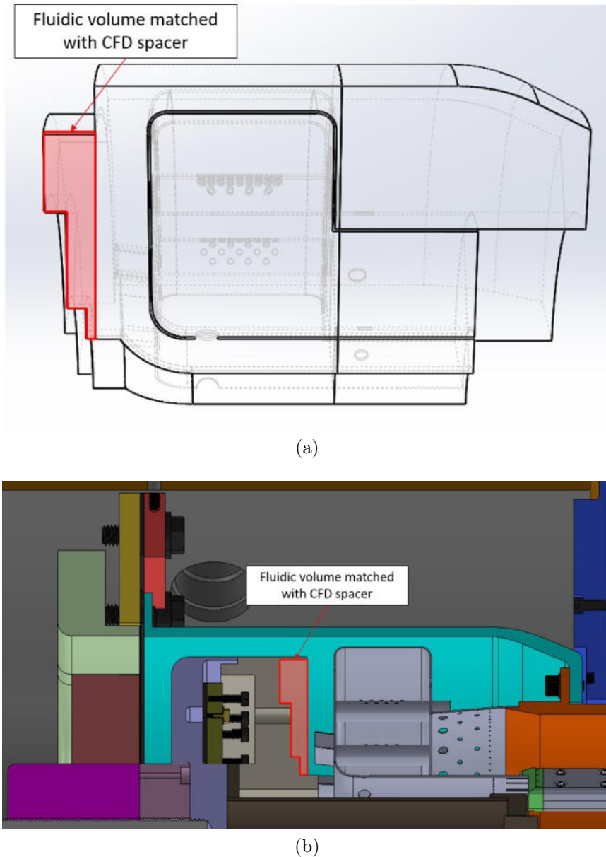
Figure 94. Combustor fluidic volume that was matched between the (a) computational and (b) experimental domains through the use of the CFD domain spacer
