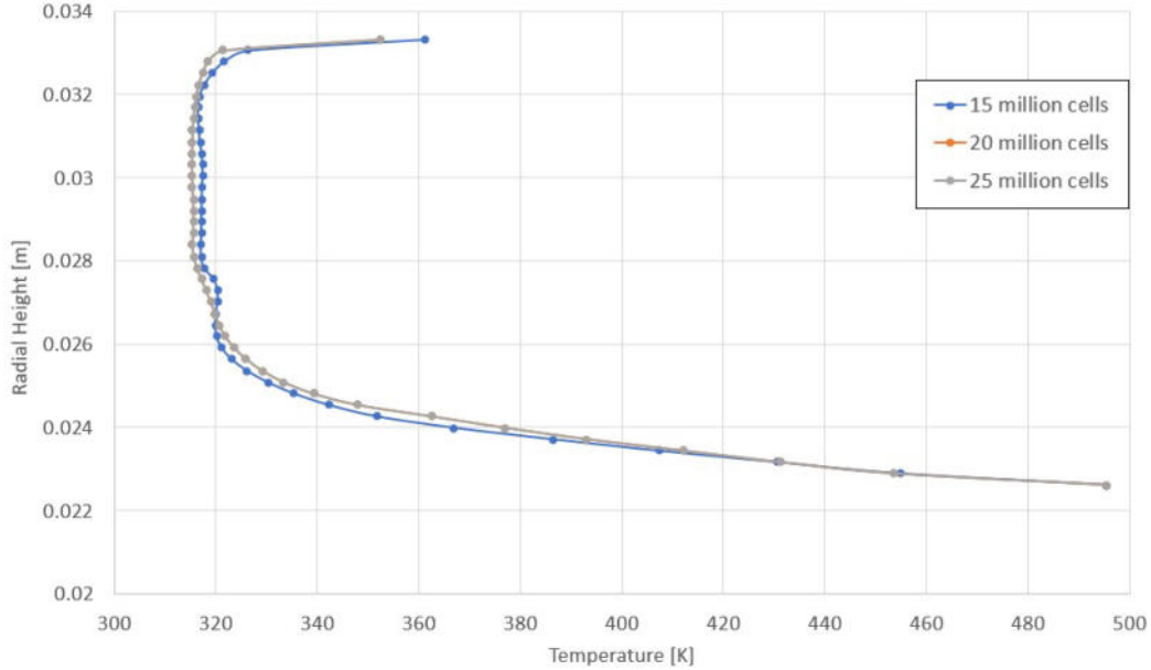
Figure 62. Temperature profile at Line 2
