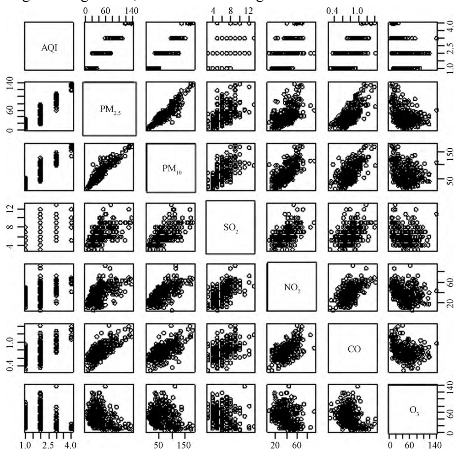
Fig. 2 Correlation scattered matrix diagram of Chengdu meteorological data
