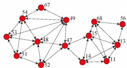
社区6的子图M 4 : 11,13,15; 11,14,15; 13,14,15; 11,13,14; 11,13,68; 14,15,47; 11,15,68; 13,15,68; 13,56,68; 49,54,67; 49,53,54; 51,53,54; 48,53,54; 48,51,54; 48,51,53; 48,49,53; 48,40,54; 48,49,52; 47,48,49; 48,51,52; 47,48,52; 47,49,52 等
