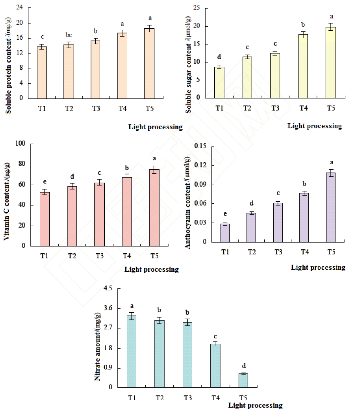
Figure 1. Effect of Light Intensity on Nutritional Quality of Purple Leaf Lettuce Seedlings
