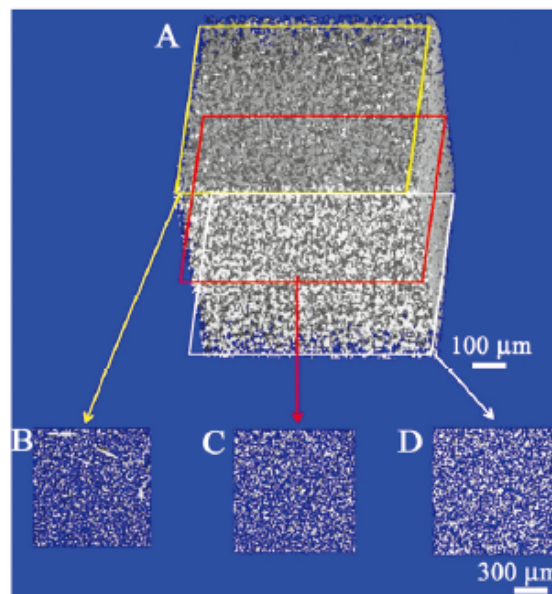
Figure 2 (A)Representative 3Dreconstructed microct image of unpurified MWCNT scaffold, and the (B) top, (C) middle and (D) bottom microct slice of the reconstructed 3-D MWCNT scaffold image [30]
