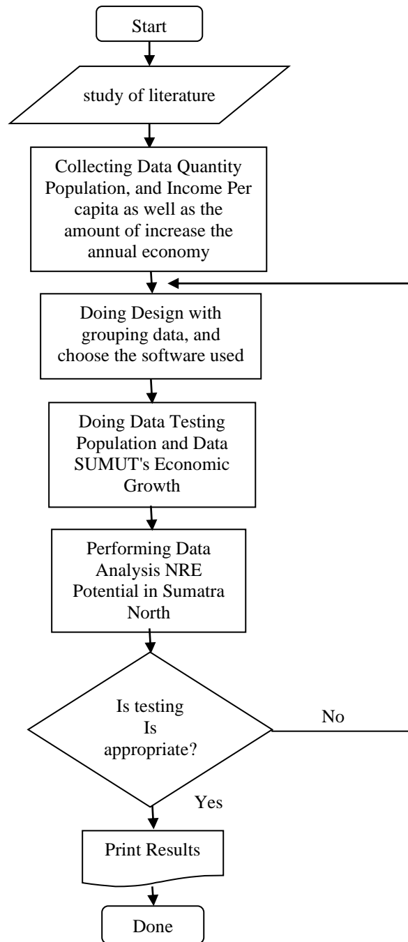
Figure 1. Research Flowchart
