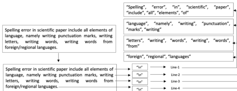
Figure 4. Tokenization in Partition of Paragraphs
