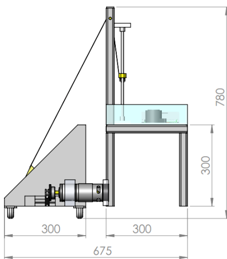
Figure 5. Side-view of the mechanical design with dimension size
