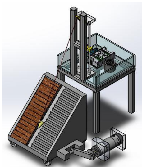
Figure 3. Perspective view of the mechanical design
