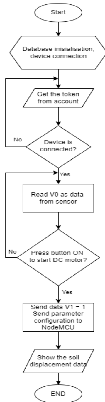
Figure 7. Blynk Platform Programming Flowchart
