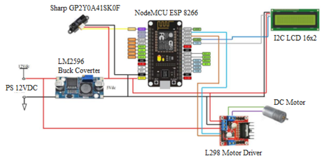
Figure 2. Wiring design of the prototype system
