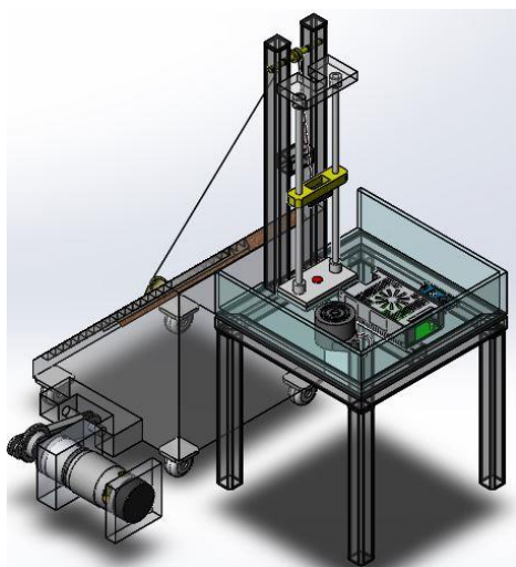
Figure 4. Back-view of the mechanical design
