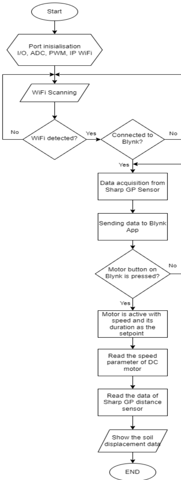
Figure 6. NodeMCU Microcontroller's Programming Flowchart
