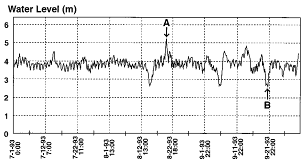
FIG. 15. Trace from Nome tide gauge for the period 1 July through 1 October 1993. Arrows A and B indicate the 20 August 1993 and 20–21 September 1993 events, respectively. Other conventions as in Fig. 3.
