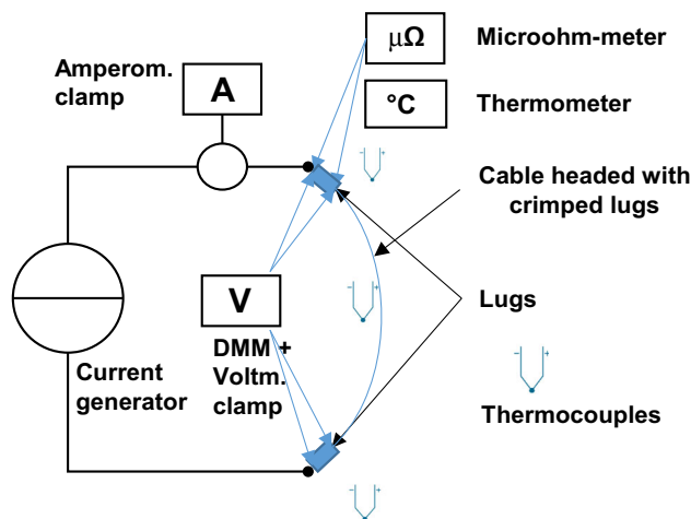
Fig. 4 Block scheme of the measurement setups for the measurements of R_{crimp} . One method is based on the direct measurement with a micro ohmmeter; the other is a voltammeter one based on the voltage measurement with a DMM and the voltmetric clamp and on the current measurement with an amperometric clamp
