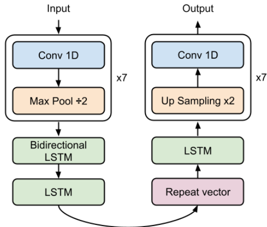
Fig. 2: Autoencoder architecture.
