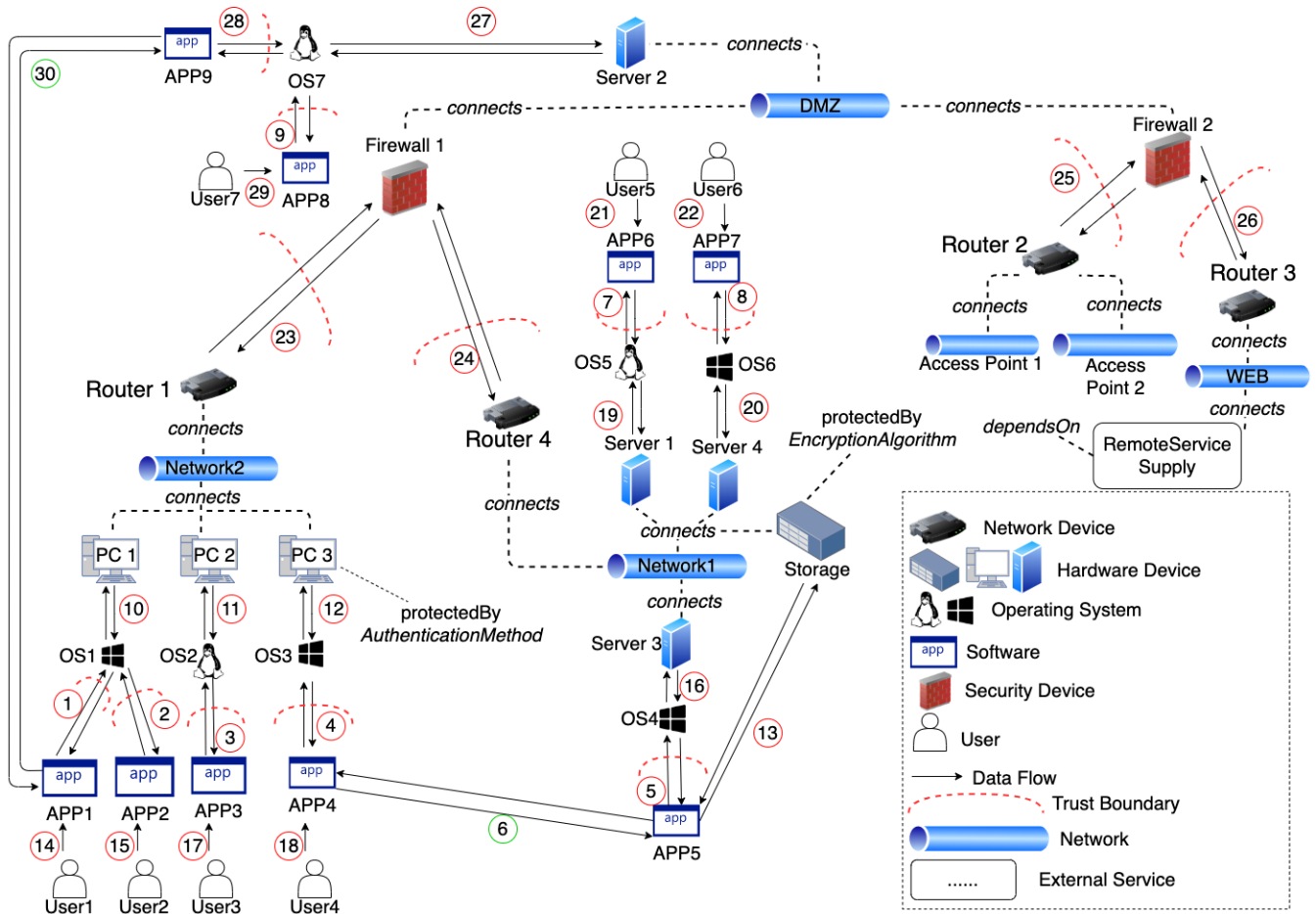
FIGURE 6. Use-case Infrastructure
